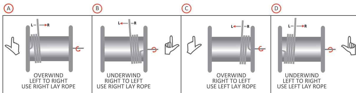
FIGURE 6 SELECTION OF LAY DIRECTION
