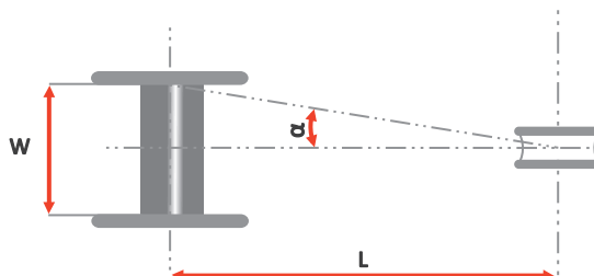
FIGURE 35 SPOOLING ARRANGEMENT
