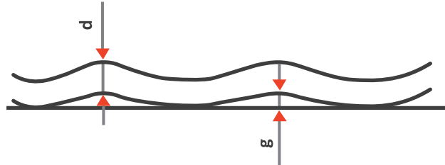
FIGURE 33 WAVINESS ASSESSMENT
