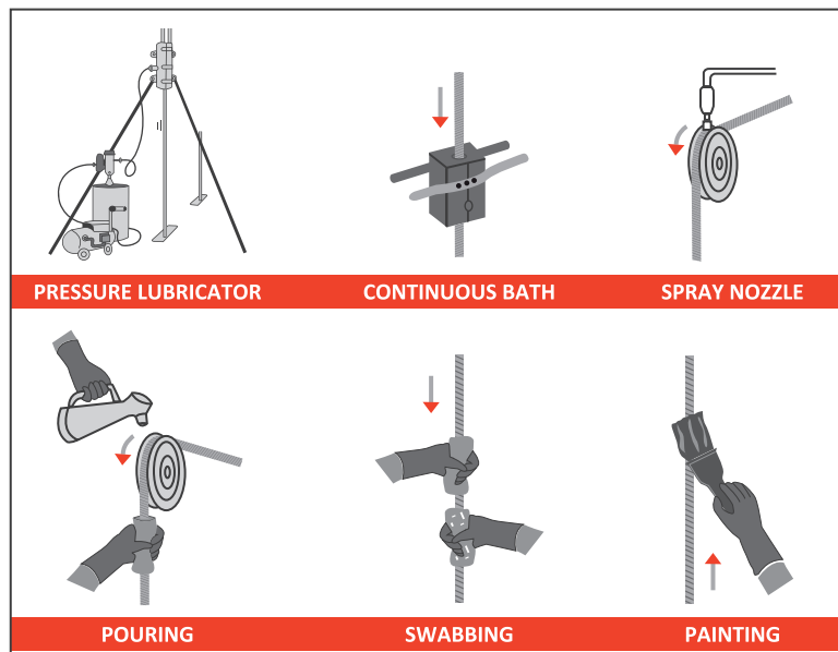
FIGURE 30 TYPICAL LUBRICATION MODES
