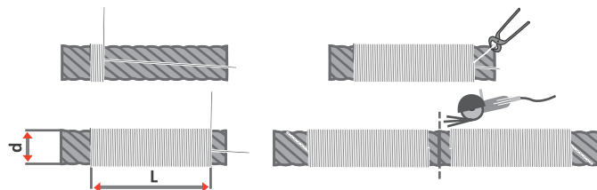
FIGURE 21 SERVING DIMENSIONS AND CONFIGURATION
