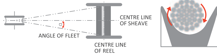
FIGURE 11 FLEET ANGLE DURING SPOOLING AND ROPE ROLLING
