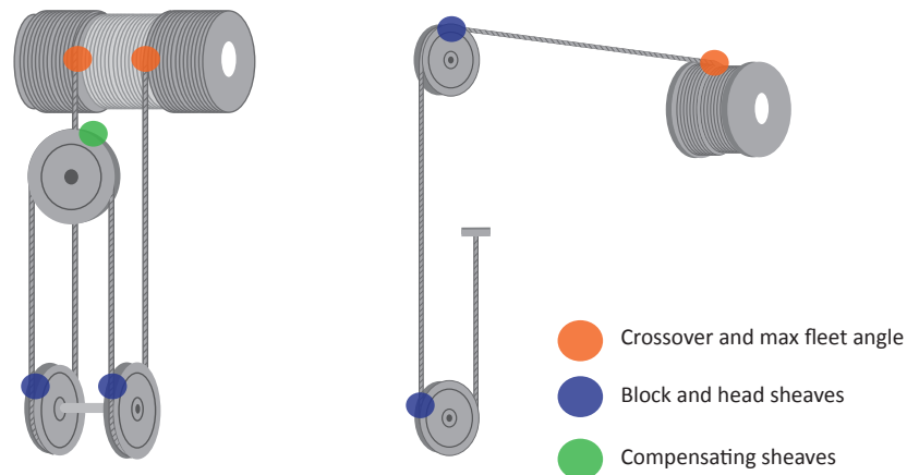
FIGURE 31 AREAS REQUIRING DETAILED INSPECTION
