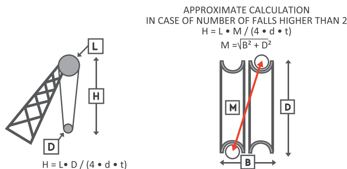
FIGURE 14 CALCULATION OF MAXIMUM LIFTING HEIGHT
