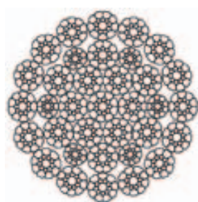
35xK19
