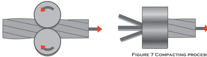
FIGURE 7 COMPACTING PROCESS THROUGH ROLLERS OR DIE
