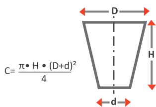
FIGURE 23 RESIN CONTENT AND CONE DIMENSIONS
