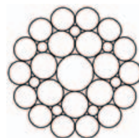
29 Filler 29F (1-7-7F-14)
