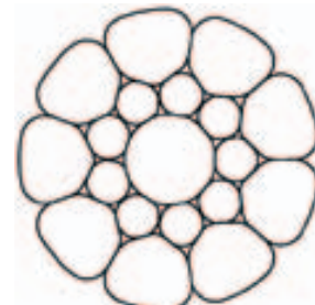
19 Seale compacted K19S (1-9-9)
