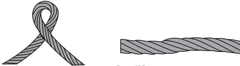
FIGURE 19 ROPE KINK AND ASSOCIATED DEFORMATION
