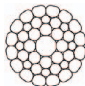
41 Warrington Seale compacted K41WS (1-8-8+8-16)
