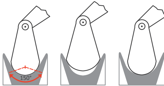
FIGURE 24 GROOVES INSPECTION: CORRECT SIZE, NARROW AND LARGE GROOVE
