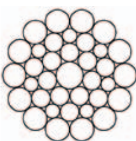
36 Warrington Seale 36WS (1-7-7+7-14)
