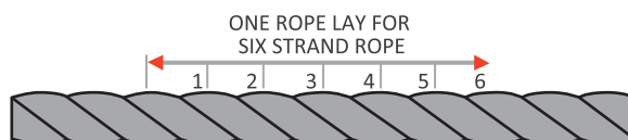
FIGURE 4 LAY LENGTH MEASUREMENT FOR A SIX STRAND ROPE
