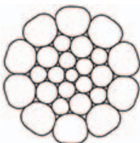
26 Warrington Seale compacted K26WS (1-5-5+5-10)
