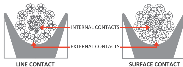
FIGURE 10 CONTACT SURFACES FOR A NON COMPACTED AND A COMPACTED ROPE
