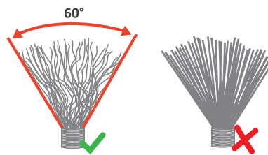
FIGURE 22 SOCKET BRUSH
