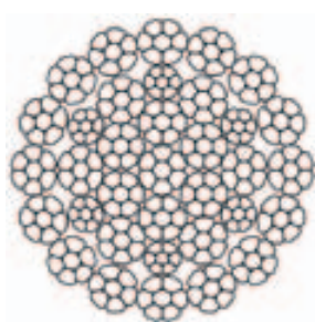
35xK7
