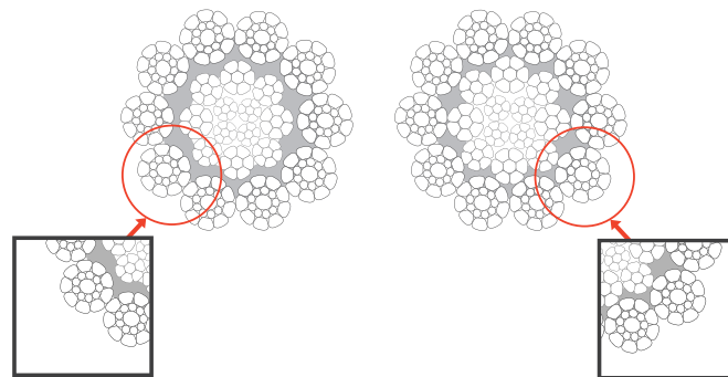
FIGURE 13 CUSHION LAYER VERSUS PLASTIC IMPREGNATED CORE
