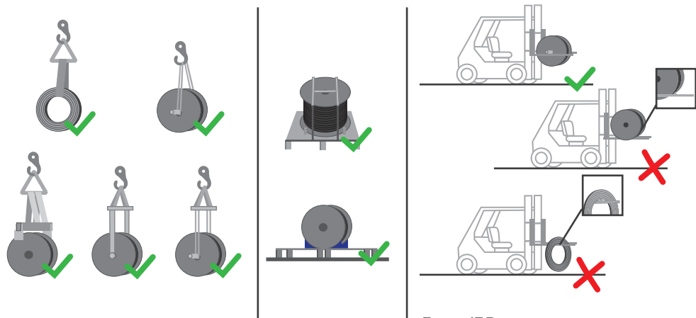
FIGURE 17 ROPE HANDLING RECOMMENDATIONS
