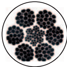
FIGURE 34 INTERNAL CORROSION
