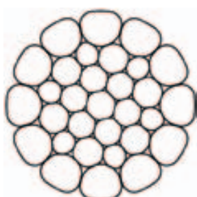
31 Warrington Seale compacted K31WS (1-6-6+6-12)
