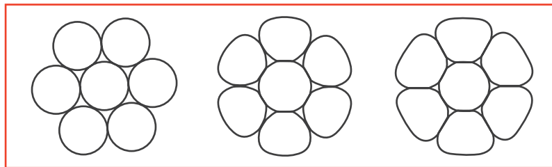
FIGURE 8 ROUND STRAND, LIGHT AND HIGH COMPACTING LEVEL
