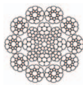
10xK19S – IWRC
