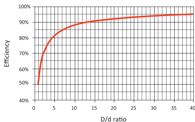
FIGURE 28 REDUCTION IN ROPE EFFICIENCY IN CASE OF BENT OVER STATIONARY COMPONENTS
