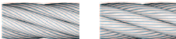
FIGURE 5 LANG LAY (LEFT FIGURE) AND REGULAR LAY (RIGHT FIGURE)
