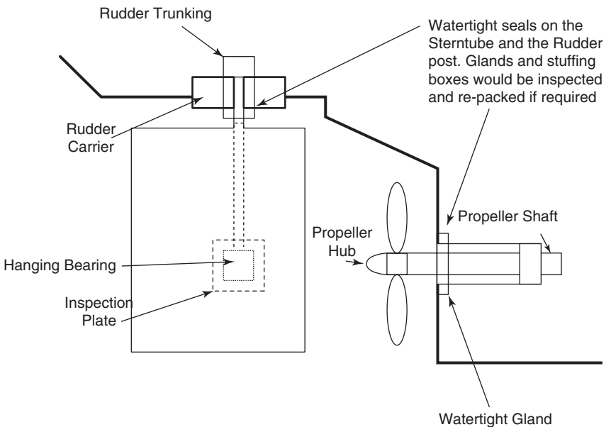
Suspended rudder – stern arrangement. Hanging/suspended rudders.
