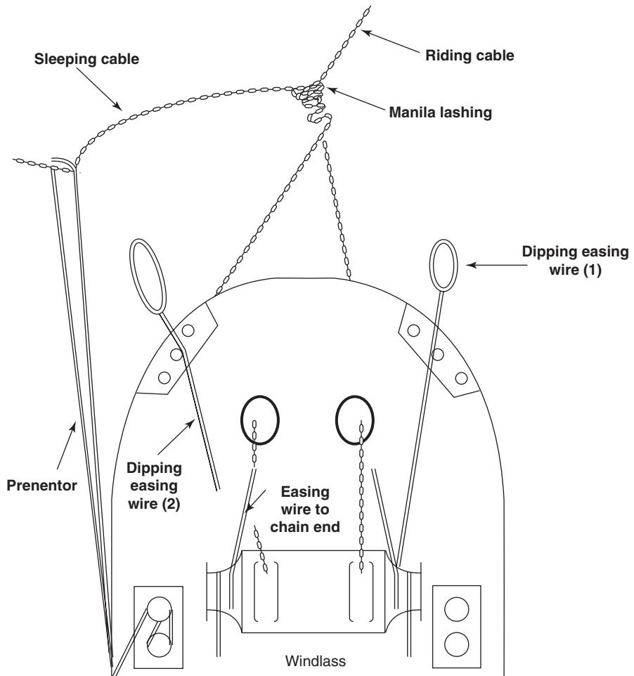
Clearing the foul hawse. Anchor securing fittings left out for clarity.
