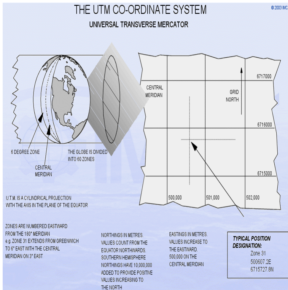
Sketch 6.1 - UTM
