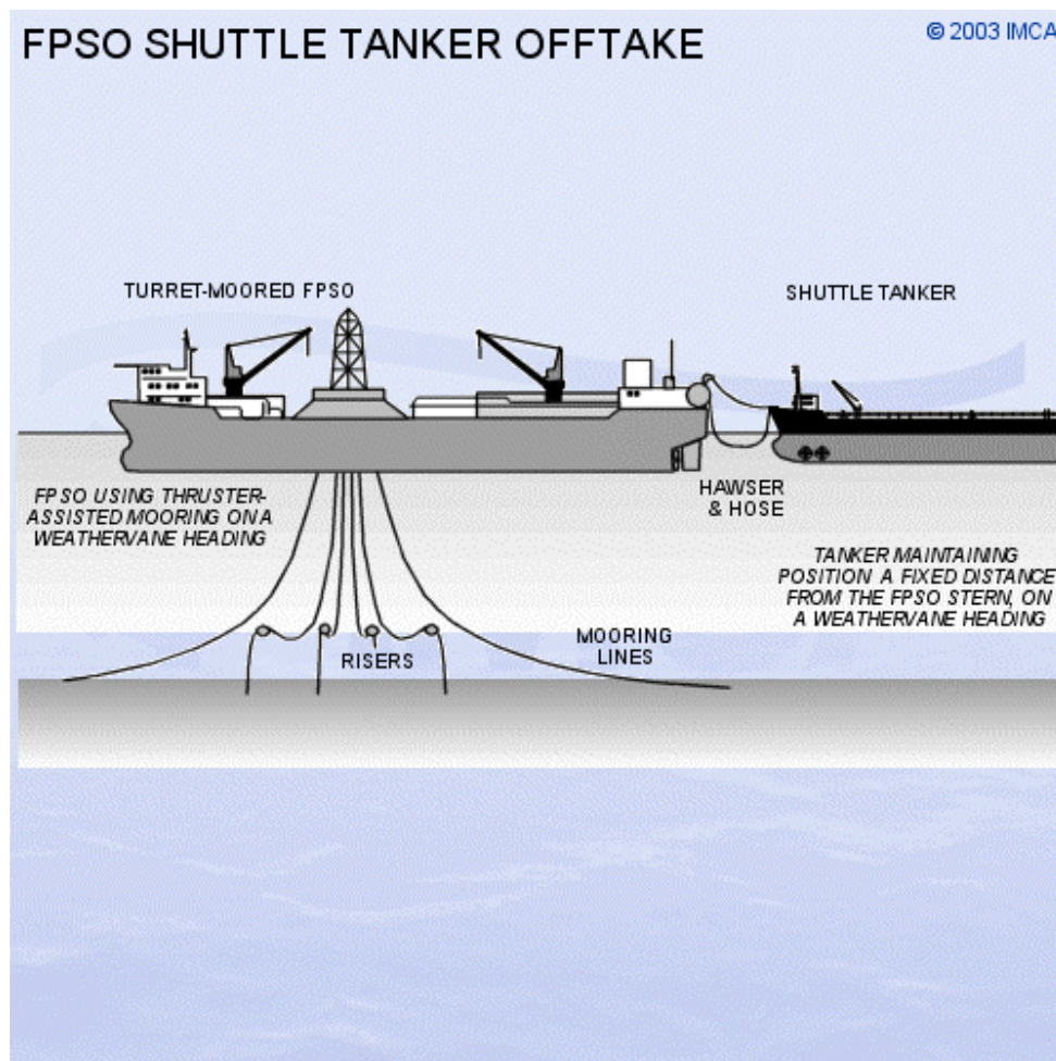
Sketch 5.13 - FPSO/shuttle tanker offtake arrangement
