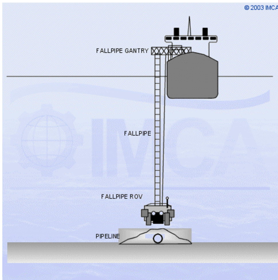
Sketch 5.7 - rockdumping
