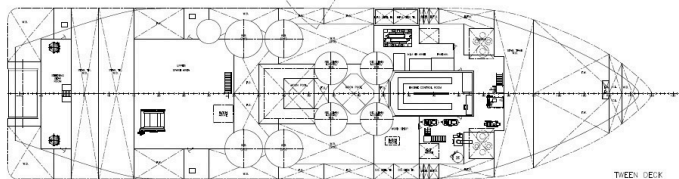
THIRD DECK
