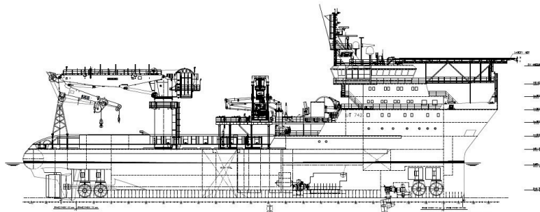
PROFILE
