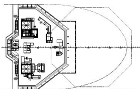
BRIDGE DECK
