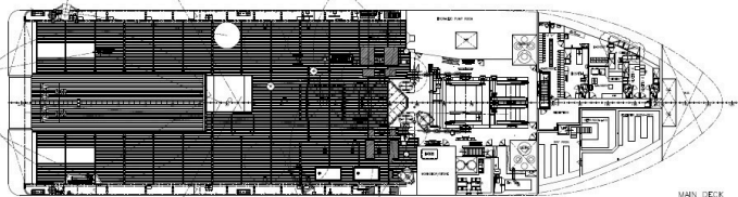
MAIN DECK
