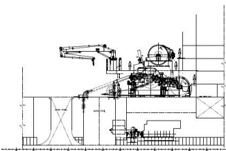
SECTION WINCHES
