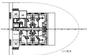
D-DECK
