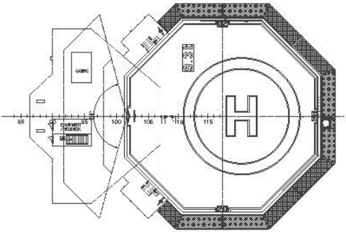
Heli deck
