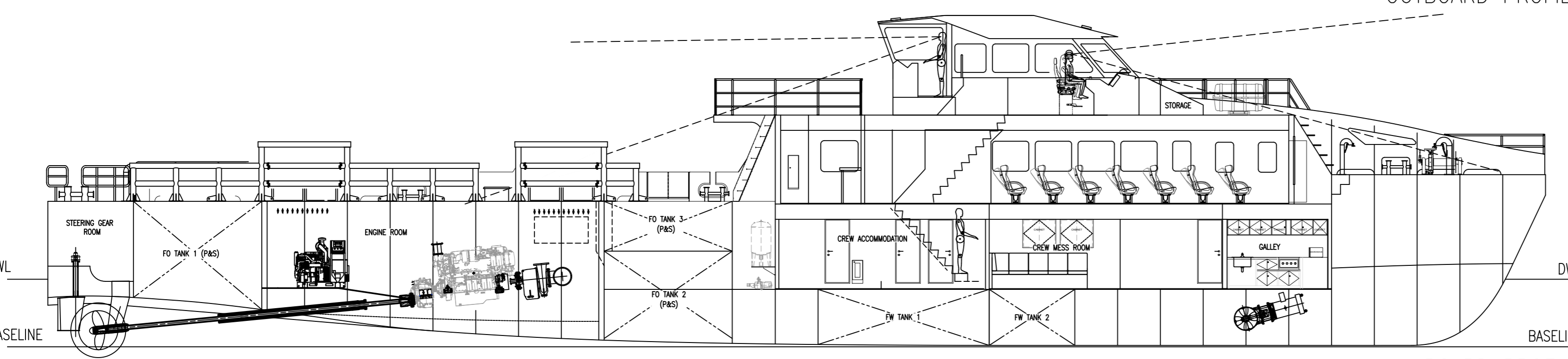
INBOARD PROFILE
