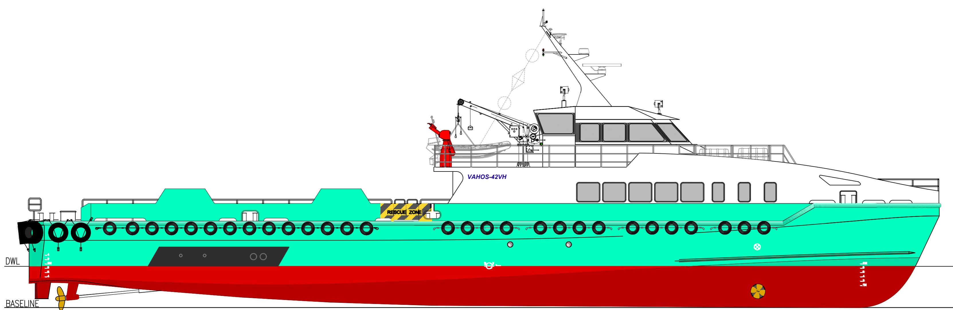
OUTBOARD PROFILE
