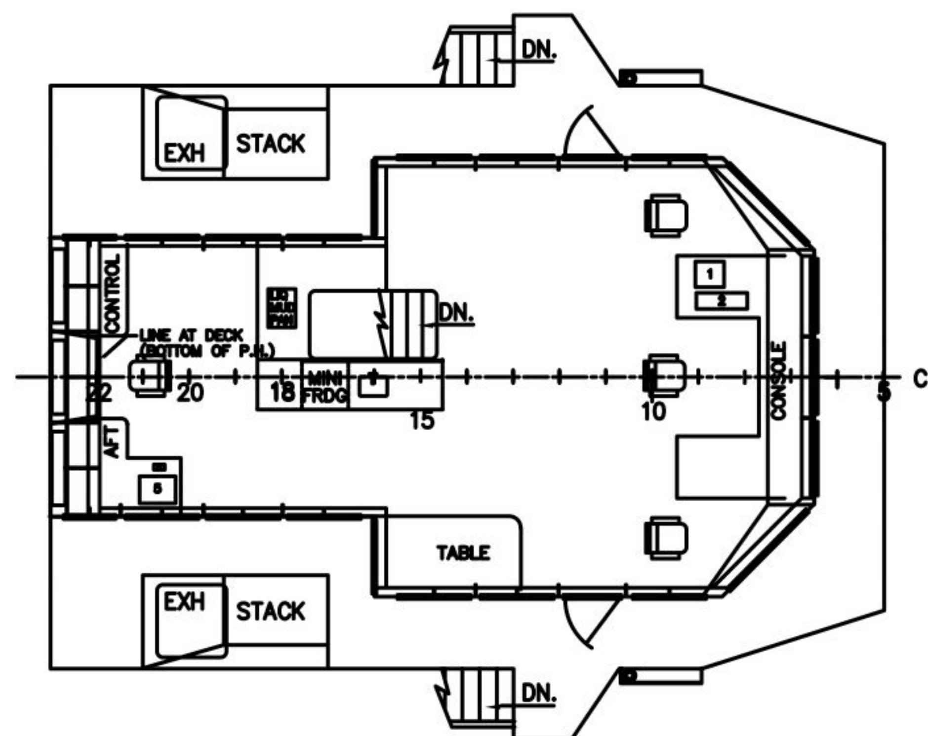
NAVIGATION DECK
