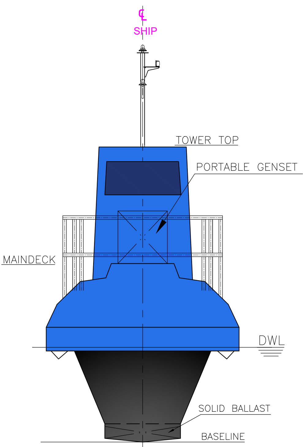
FRONT VIEW
