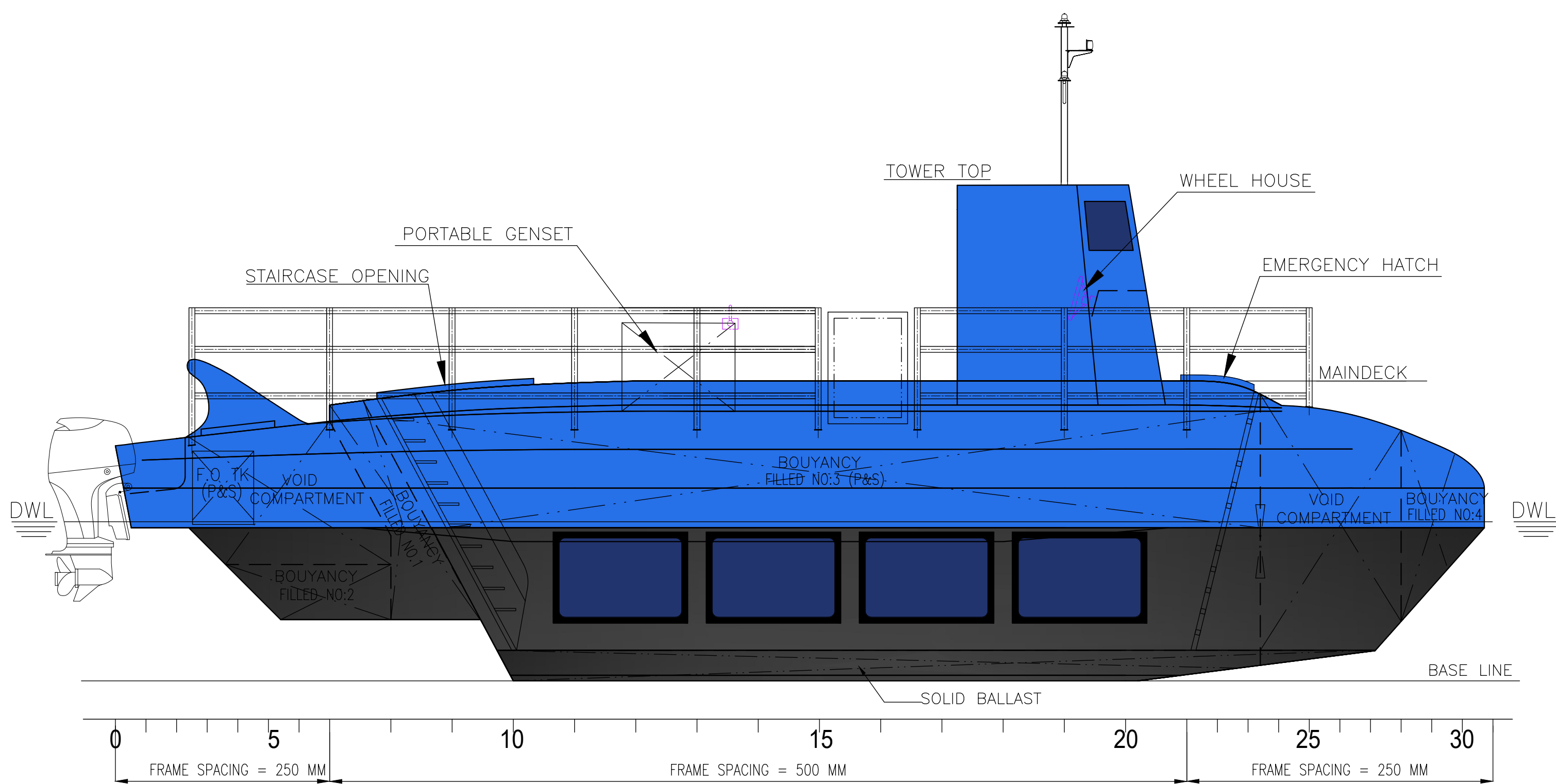
PROFILE
