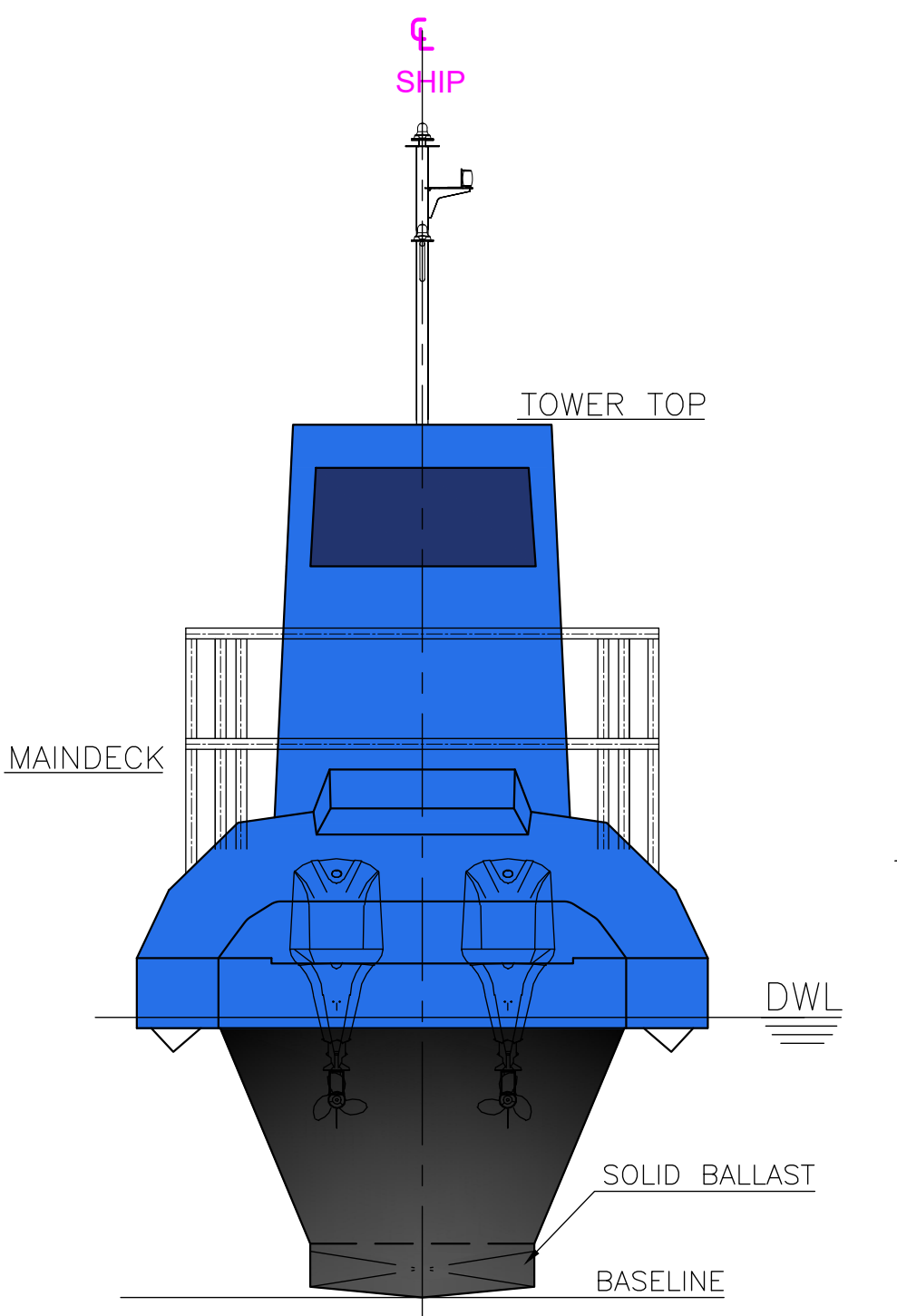
AFT VIEW
