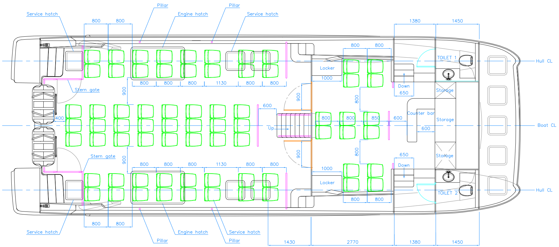
DECK PLAN 70 Seats
