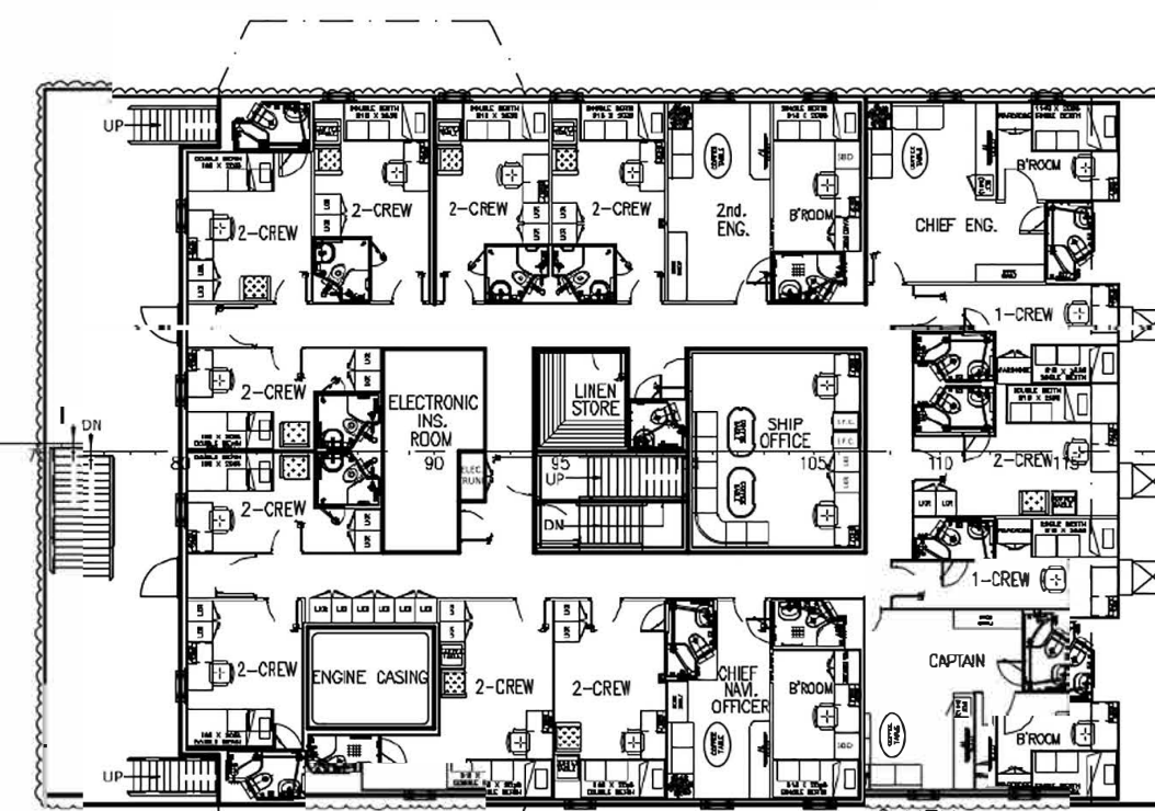
OFFICERS DECK PLAN
