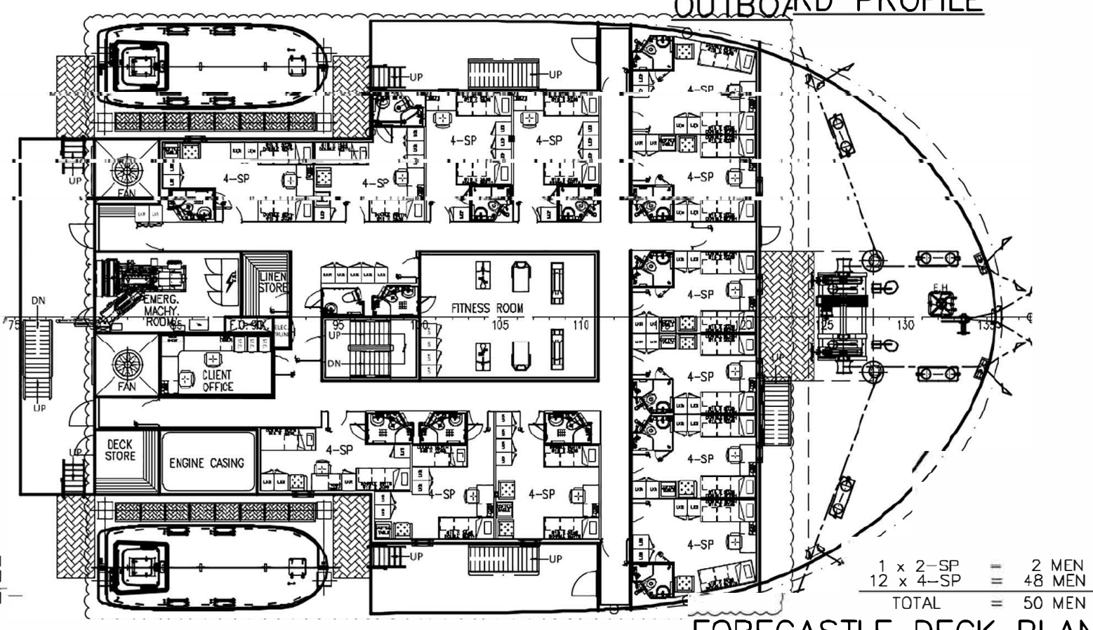
FORECASTLE DECK PLAN
