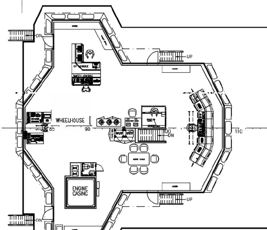
BRIDGE DECK PLAN
