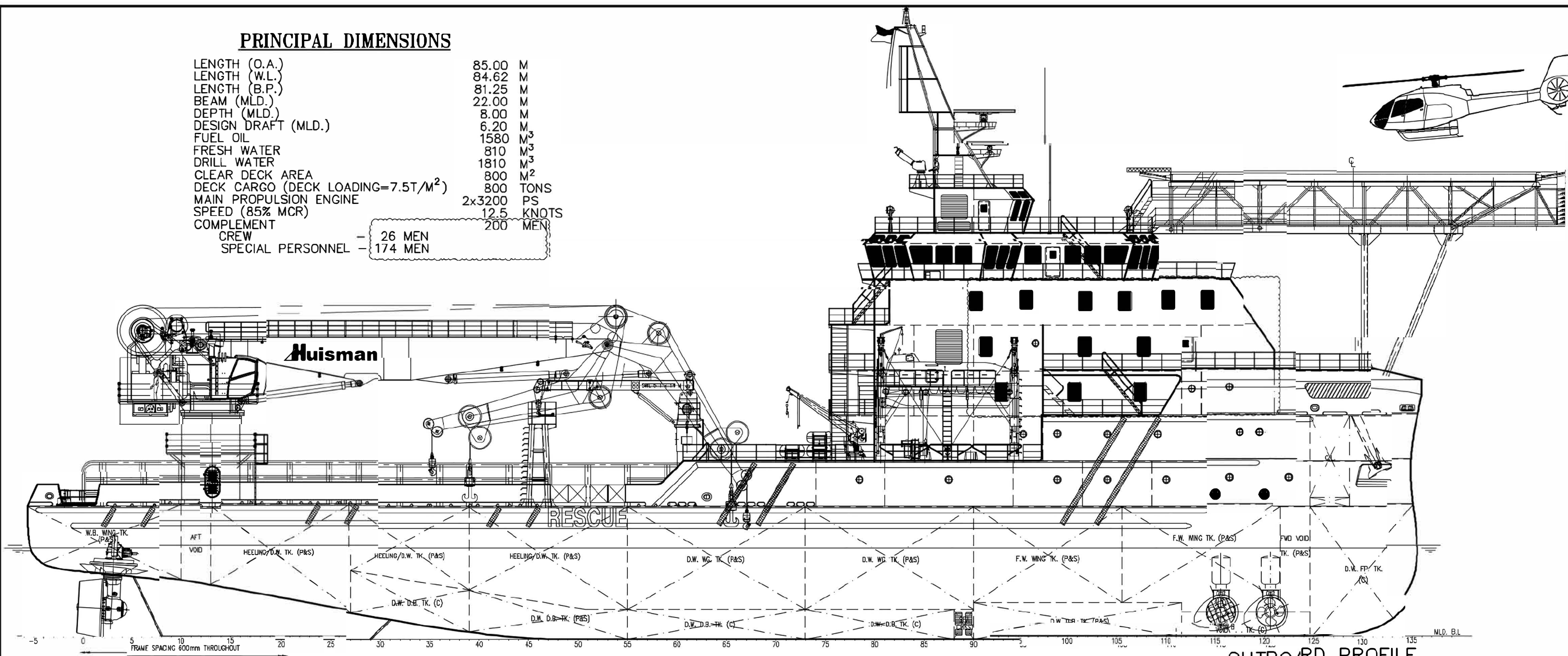
OUTBOARD PROFILE
