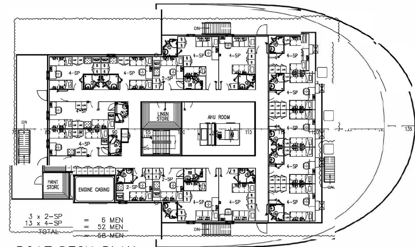
BOAT DECK PLAN
