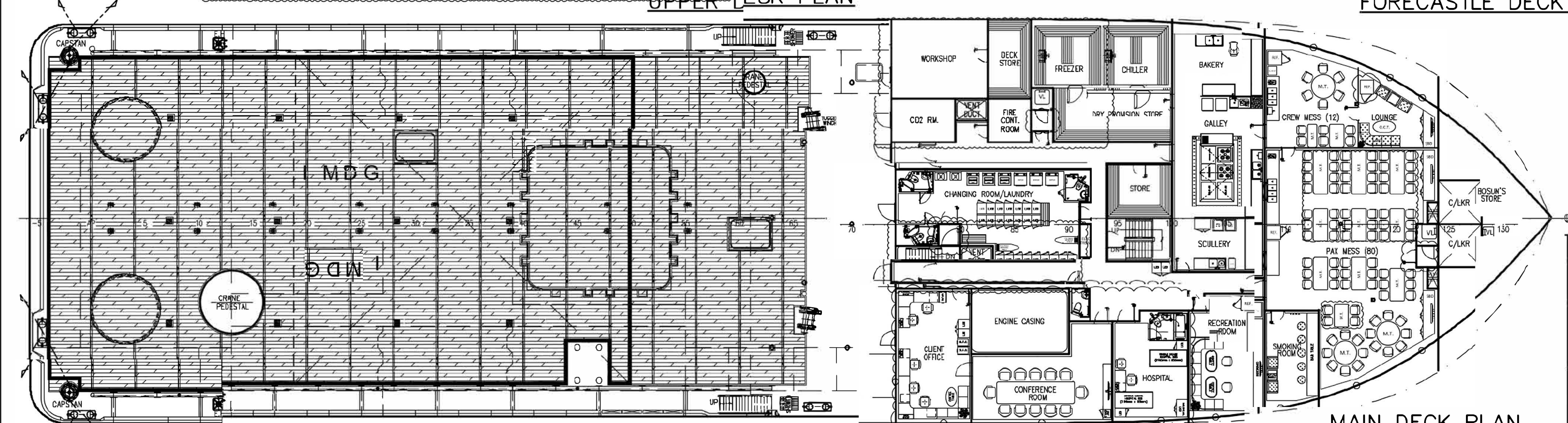
MAIN DECK PLAN
