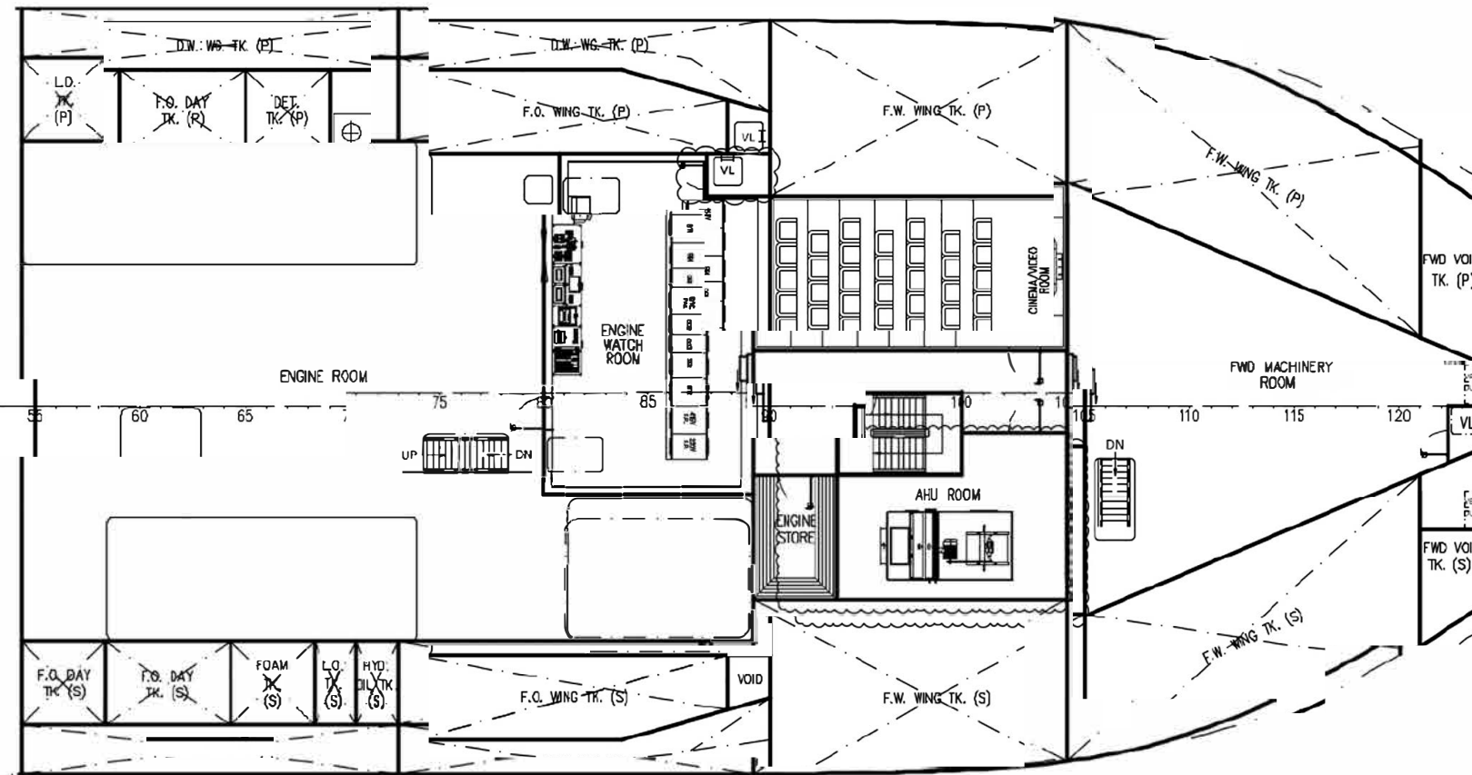
TWEEN DECK PLAN
