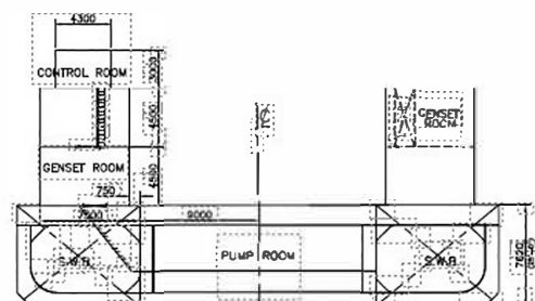
SECTION TWO PUMP ROOM
