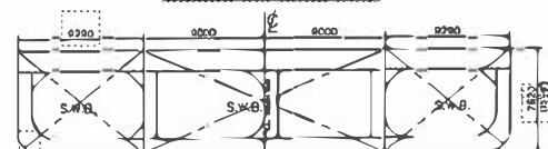
TYPICAL TRANS. SECTION:
