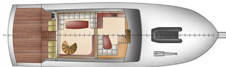
MAIN DECK
