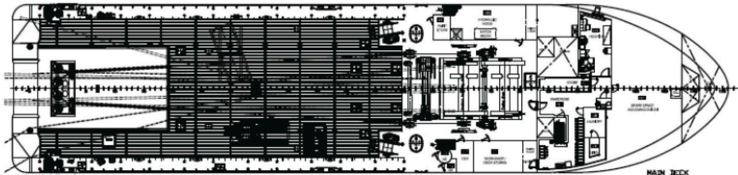
MAIN DECK
