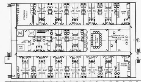
ACCOMMODATION LEVEL - 02 214x MEN, 342 MEN, 95 MEN = 95 MEN
