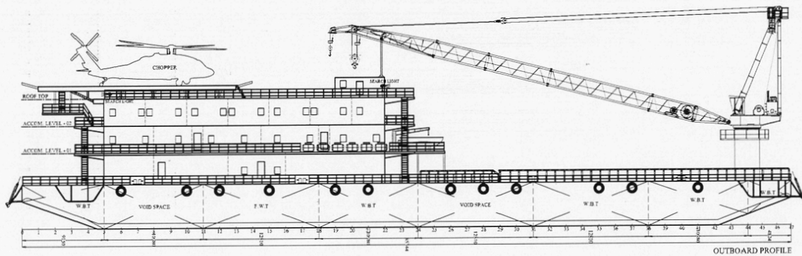
OUTBOARD PROFILE
