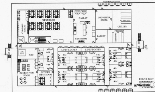
ACCOMMODATION LEVEL - 01 144x MEN = 56 MEN
