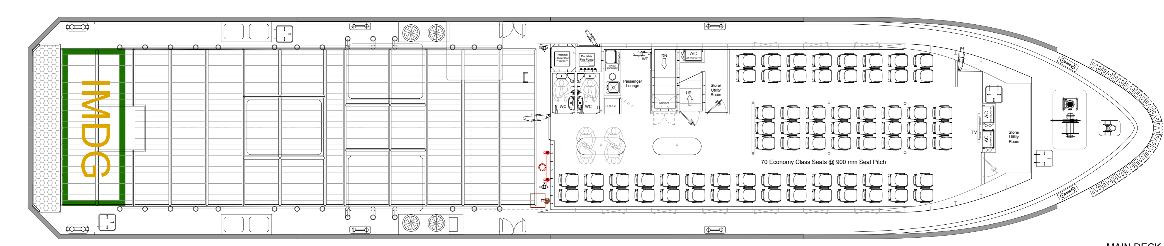
MAIN DECK
