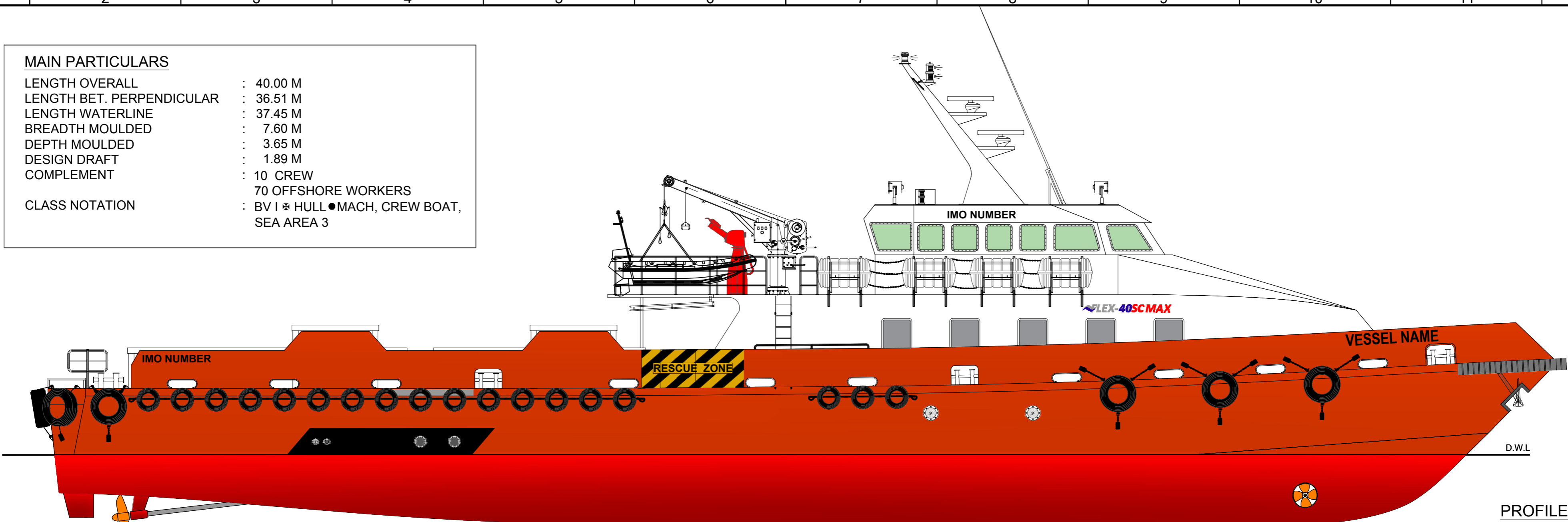
PROFILE
