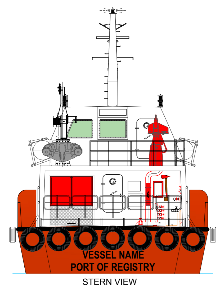
STERN VIEW
