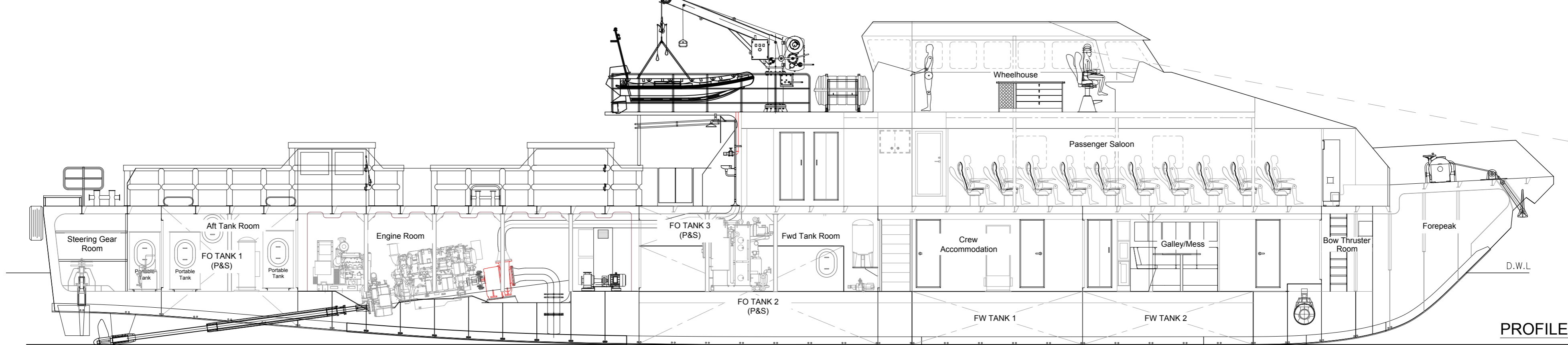
PROFILE
