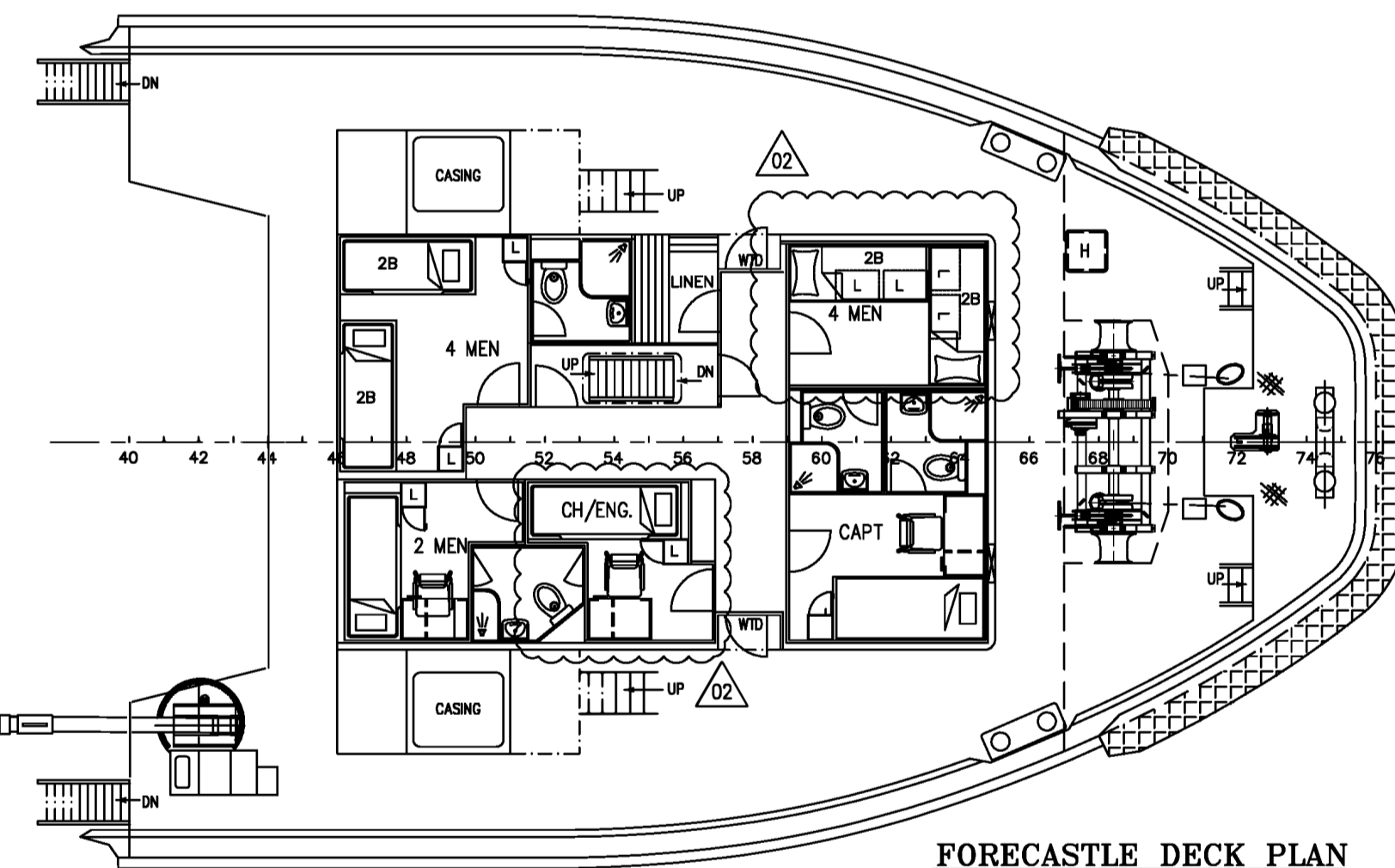
FORECASTLE DECK PLAN
