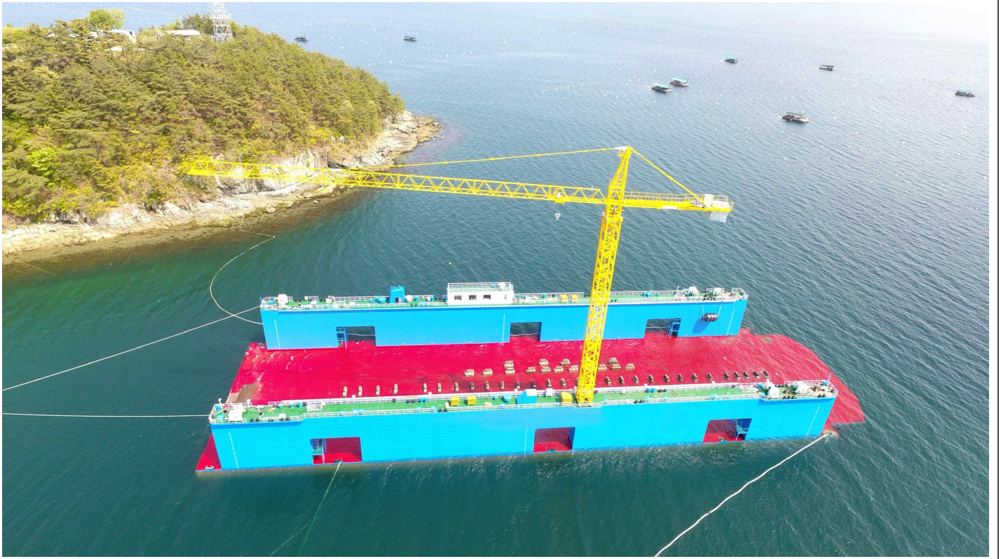
Floating Dock Photo (3)
