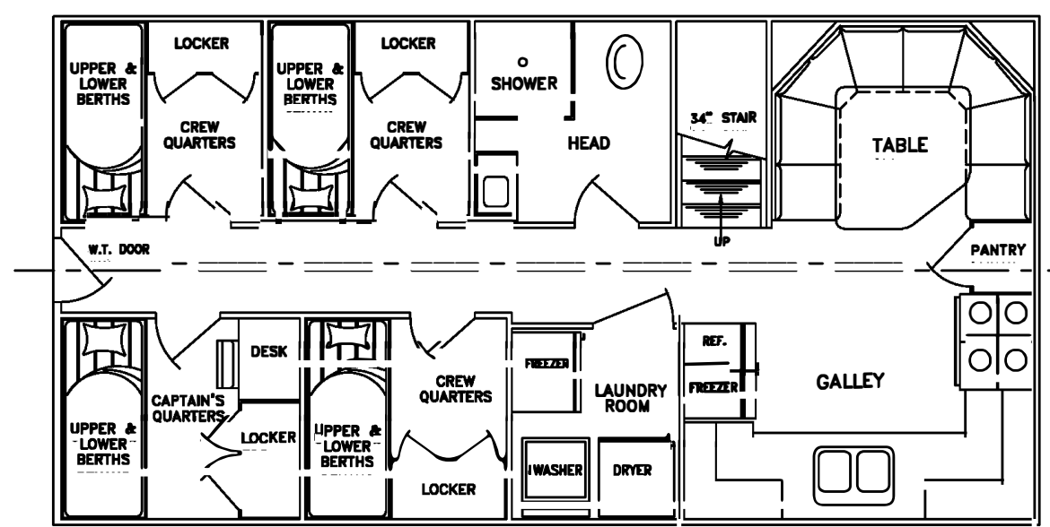
23 BELOW DECK PLAN 11
