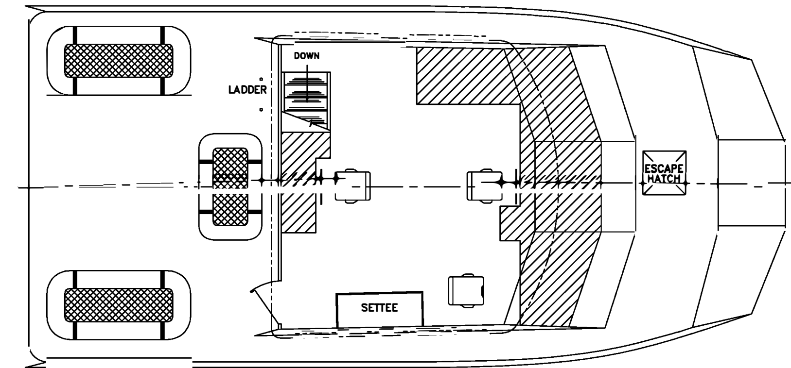
PILOT HOUSE PLAN
