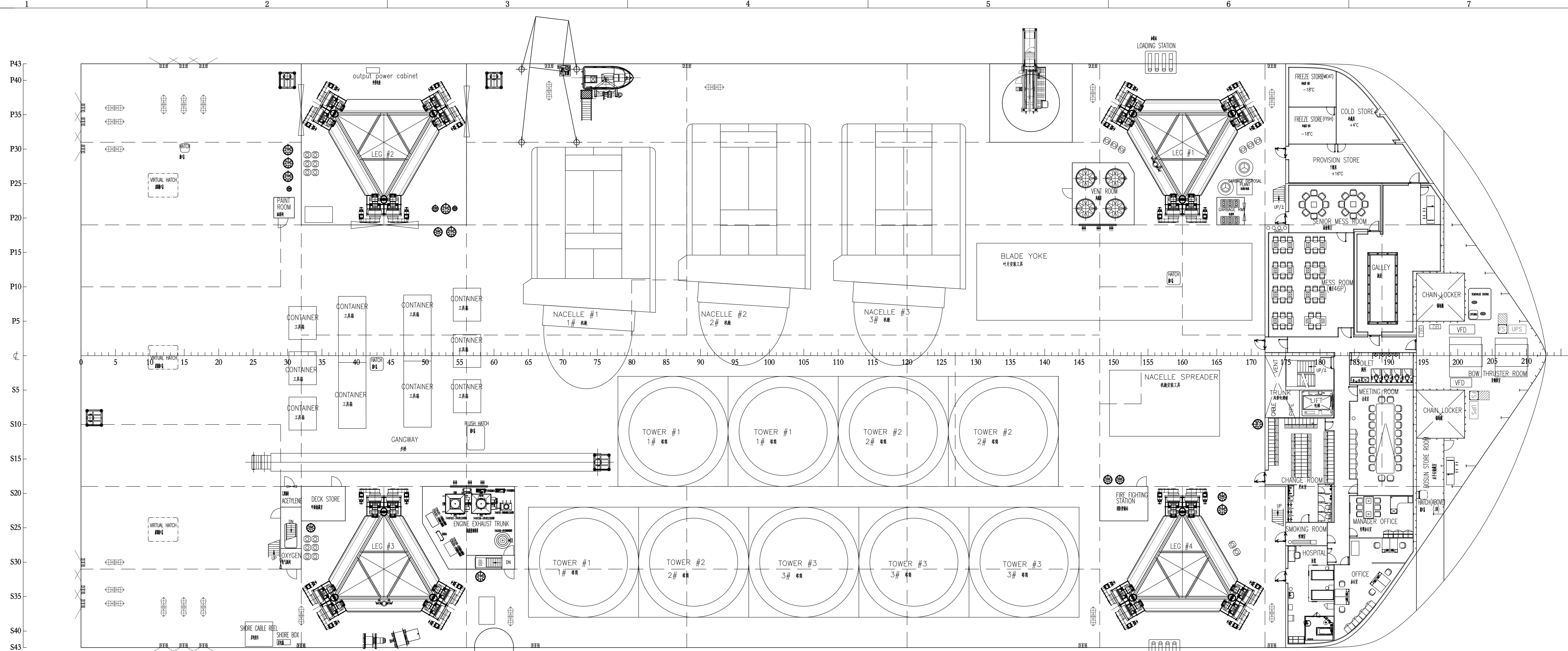
MAIN DECK / 主甲板 EL. 11.00m ABL.
