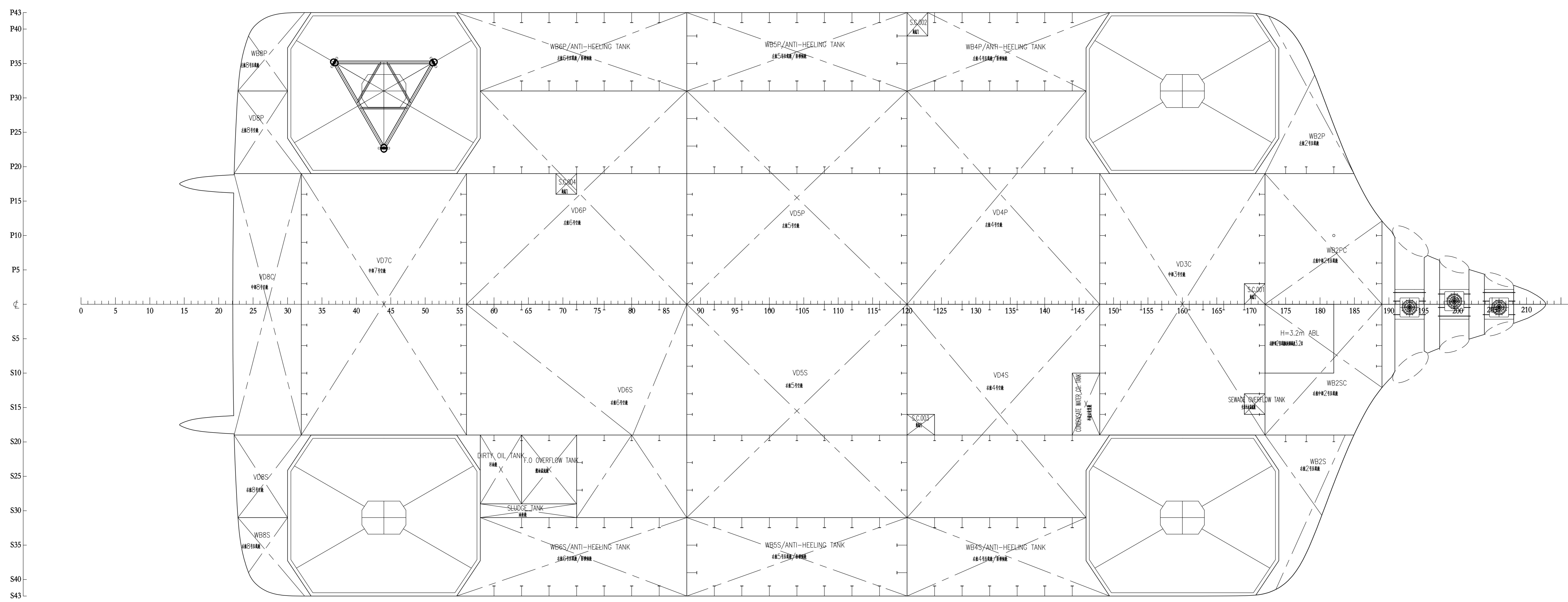
BELOW TANK TOP / 双层底
