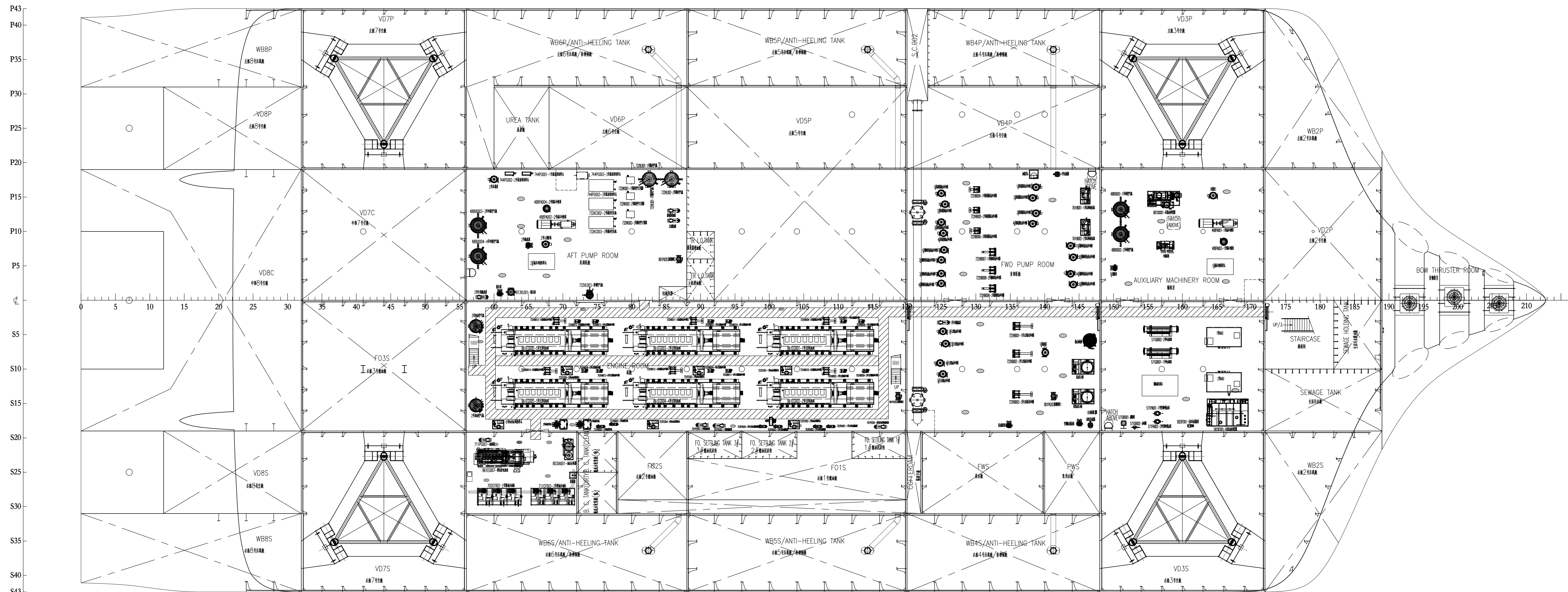
TANK TOP / 内底甲板 EL. 2.00m ABL.
