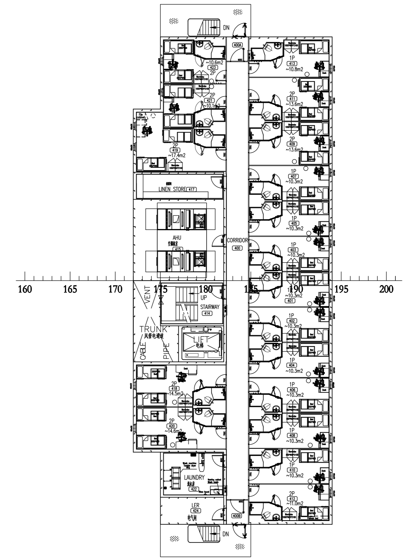
C DECK / C 甲板 EL. 20.20m ABL. 1X10=10P 2X8=16P
