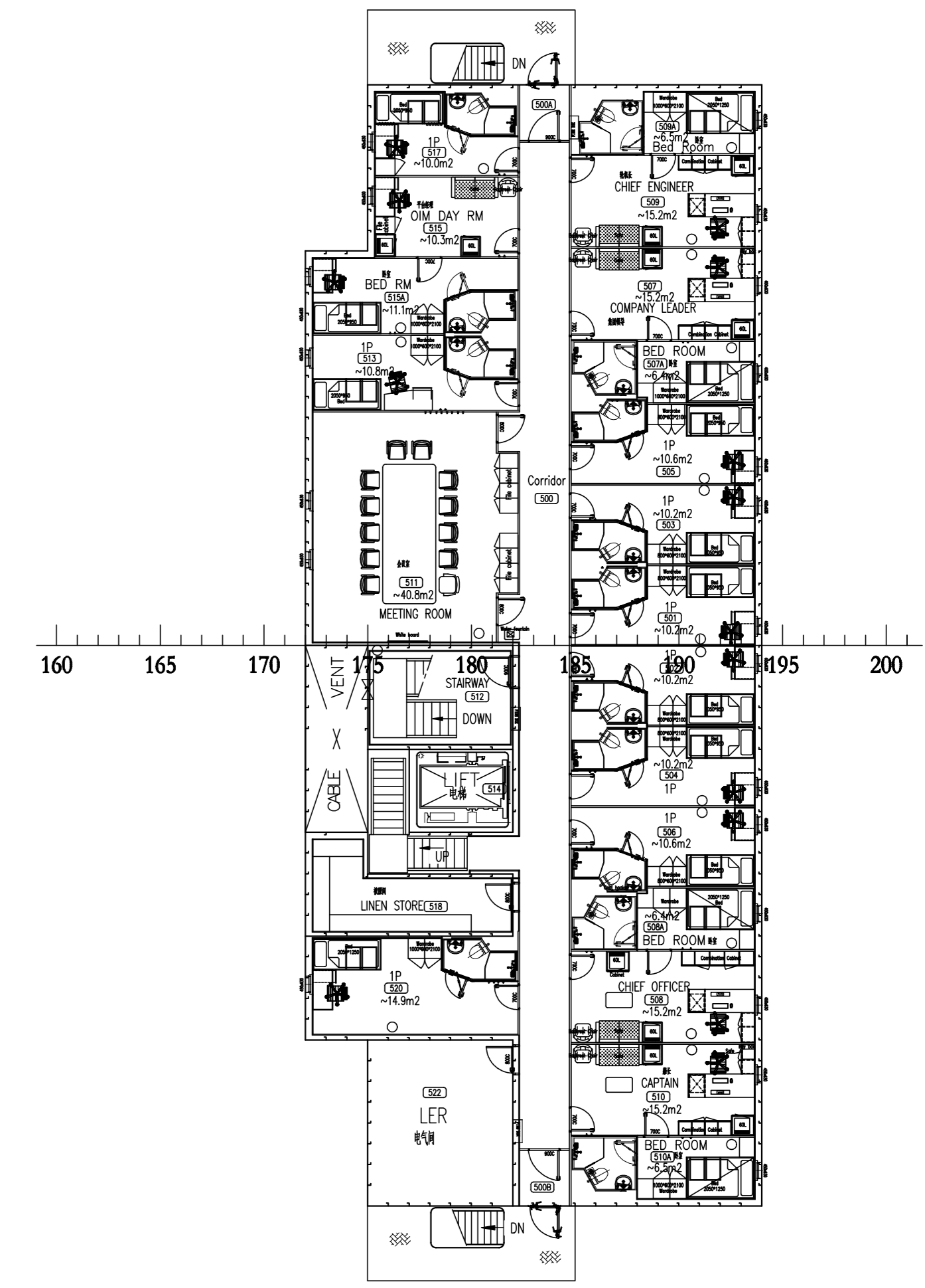
D DECK / D 甲板 EL. 23.20m ABL. 1X5=5P(SUITE) 1X9=9P
