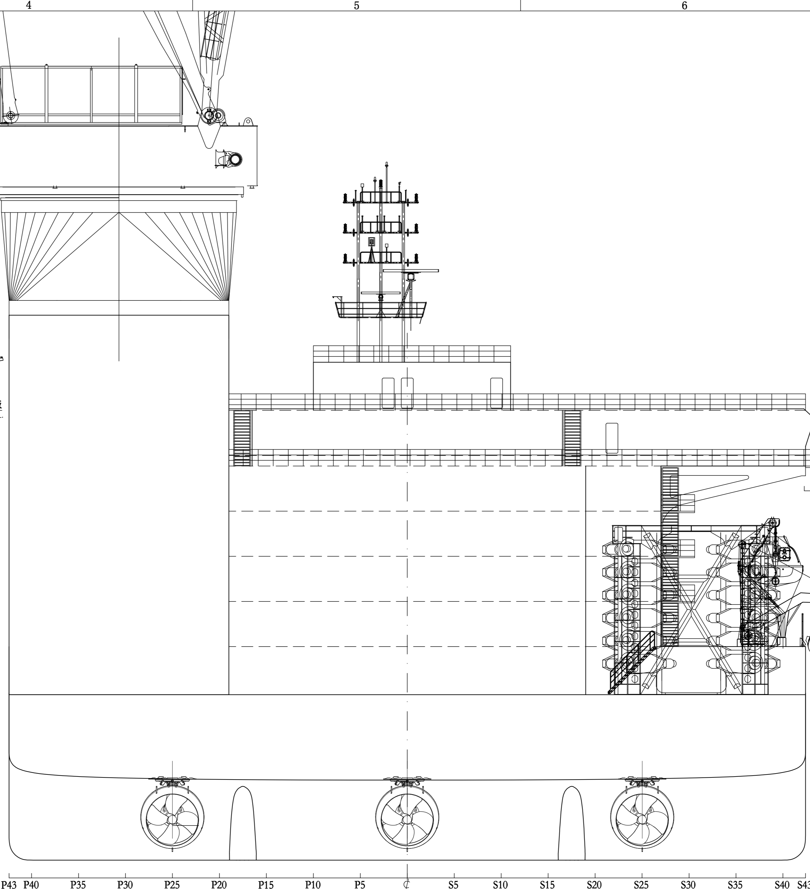
AFT VIEW / 尾视图 LOOKING FWD / 向首看
