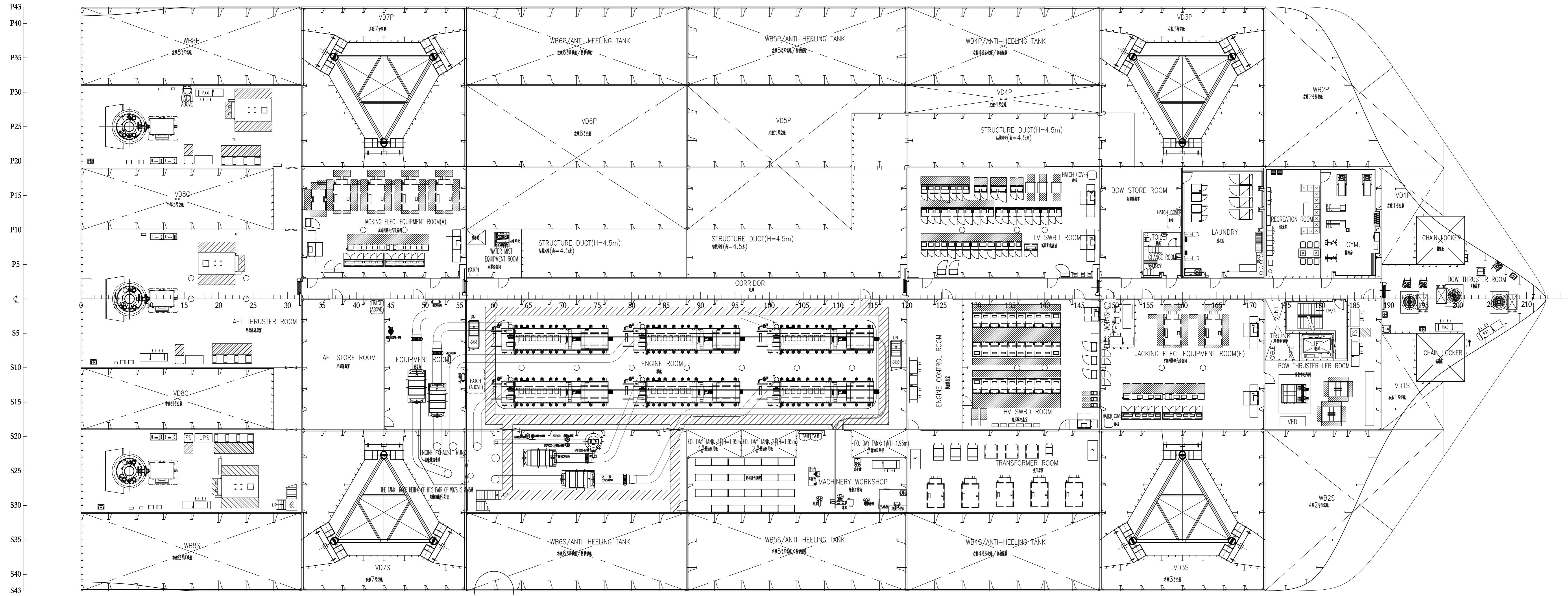
TWEEN DECK / 间甲板 EL. 6.50m ABL.
