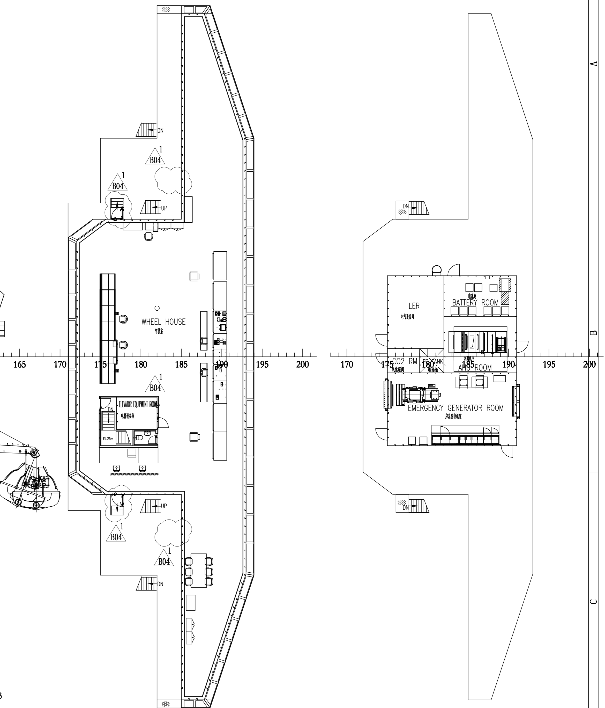
BRIDGE DECK / 驾驶甲板 EL. 26.20m ABL. COMPASS DECK / 罗经甲板 EL. 29.90m ABL.
