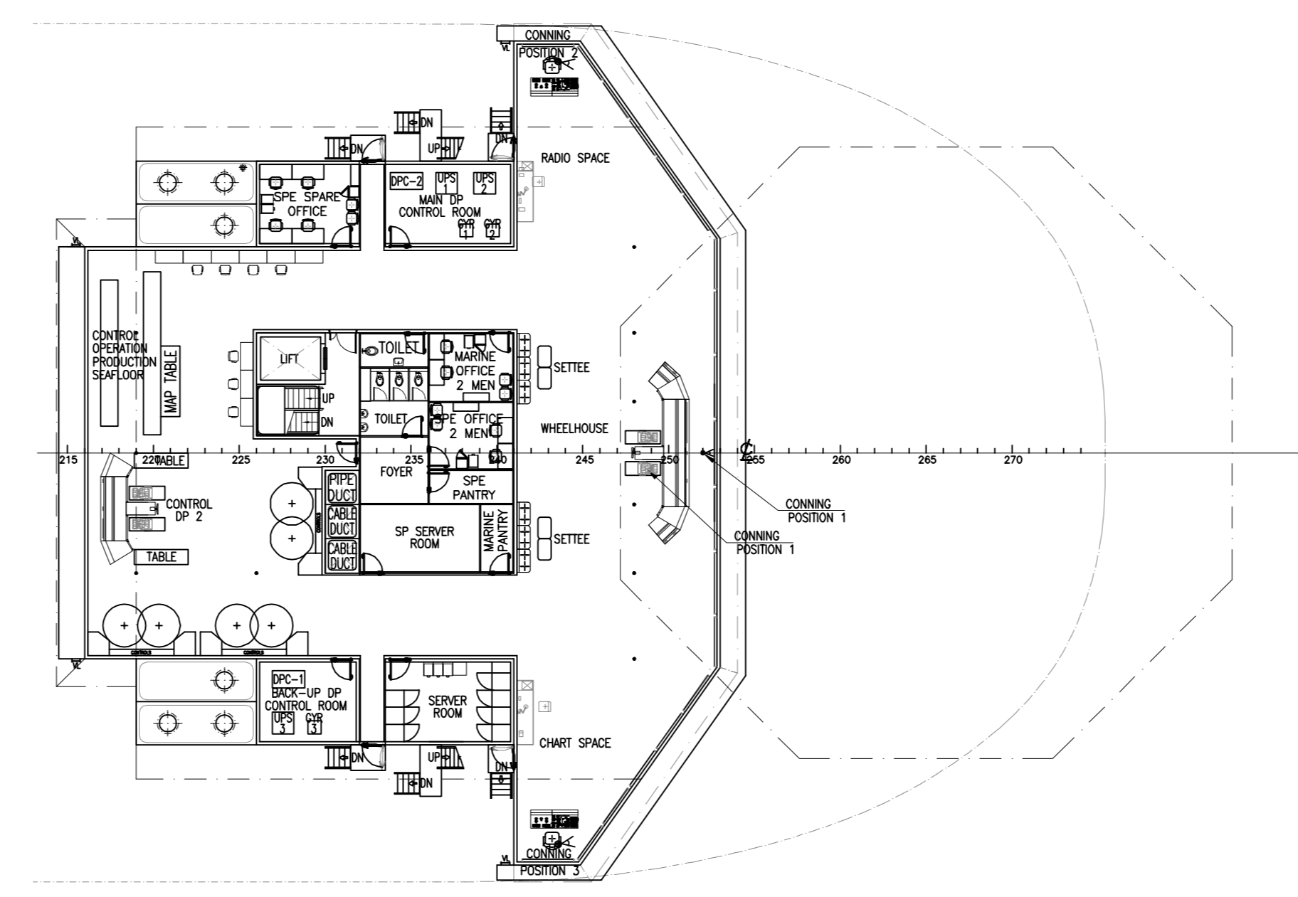
WHEELHOUSE DECK PLAN
