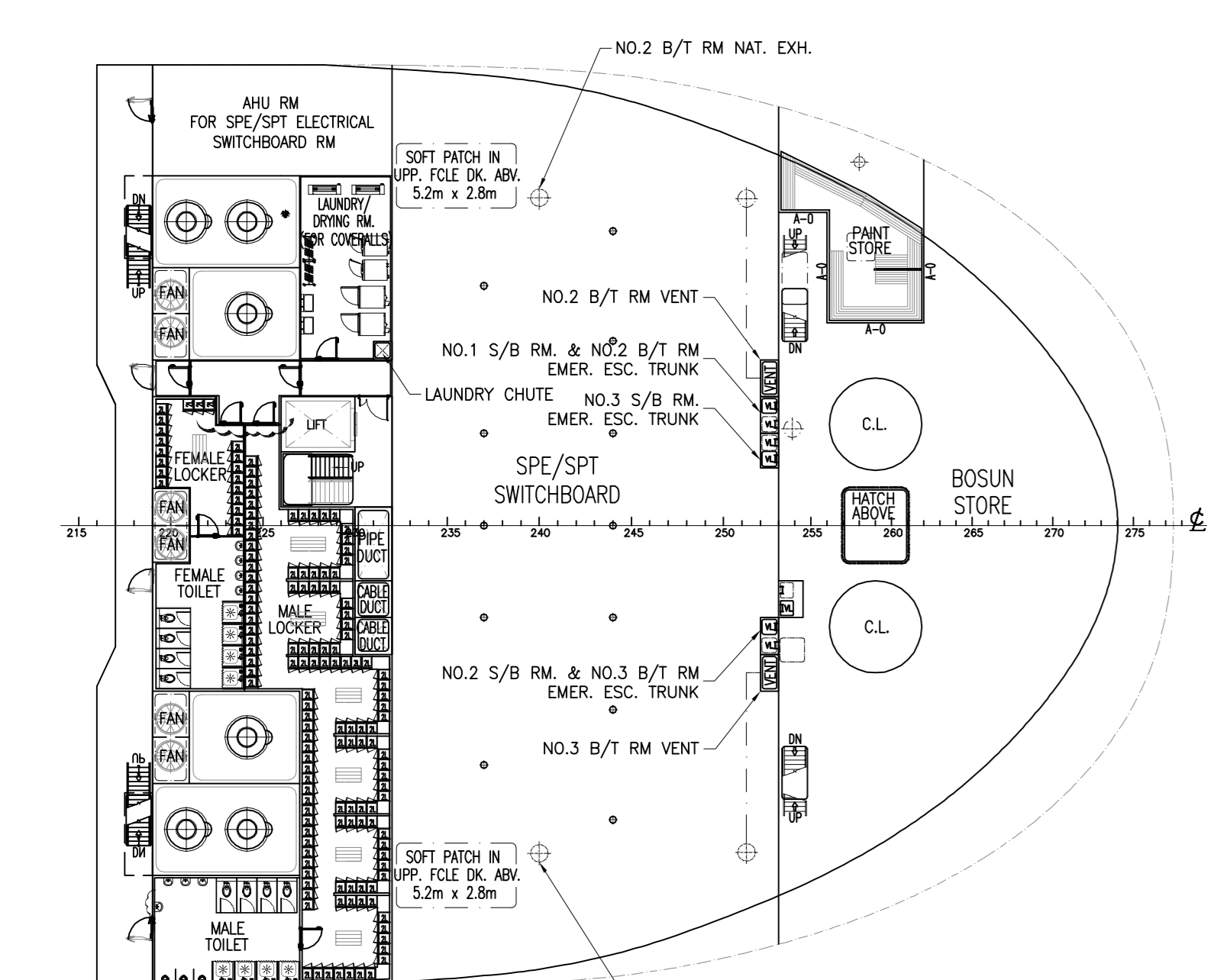
FORECASTLE DECK PLAN
