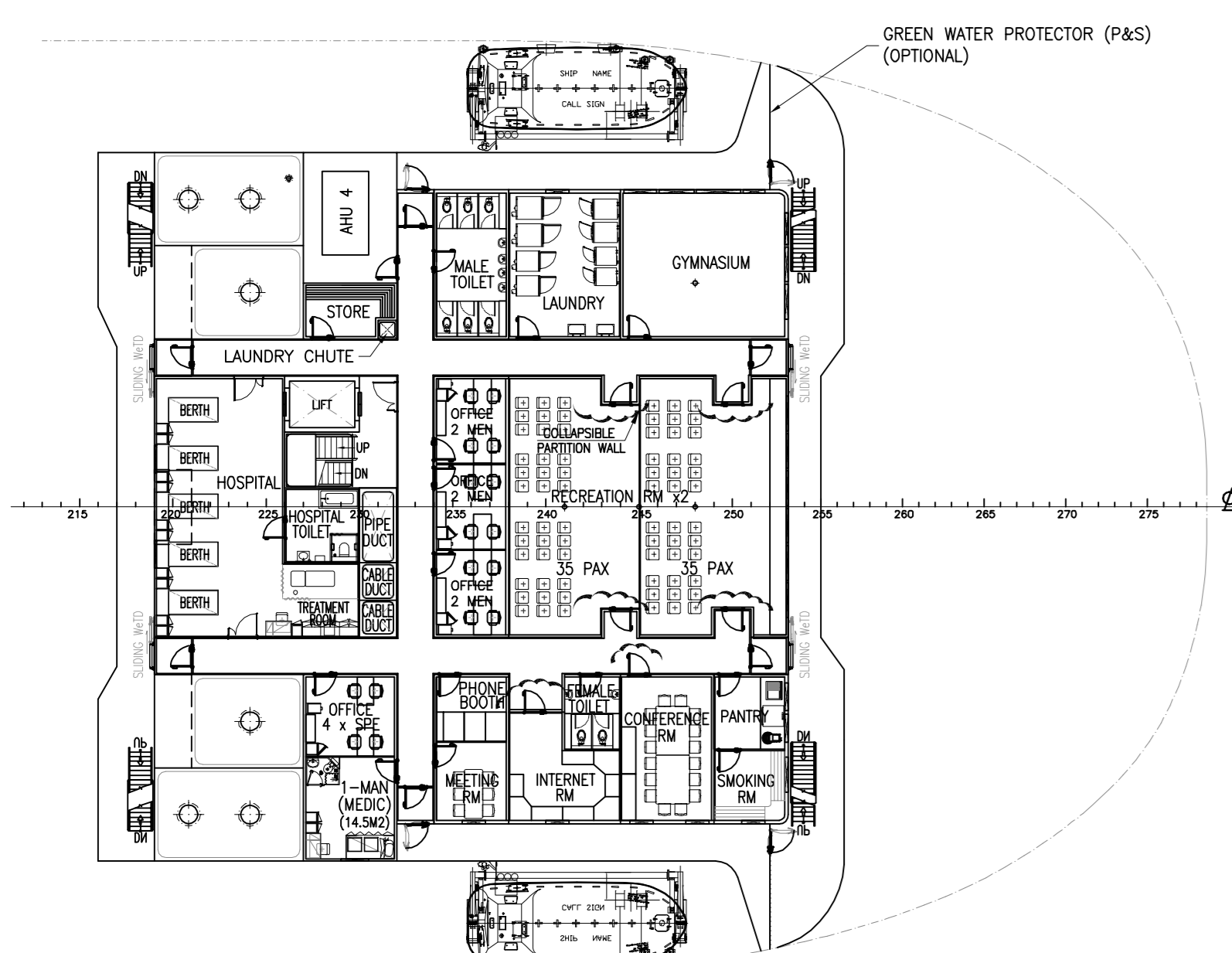
ACCOMMODATION DECK A 1 X 1-MAN= 1 MAN
