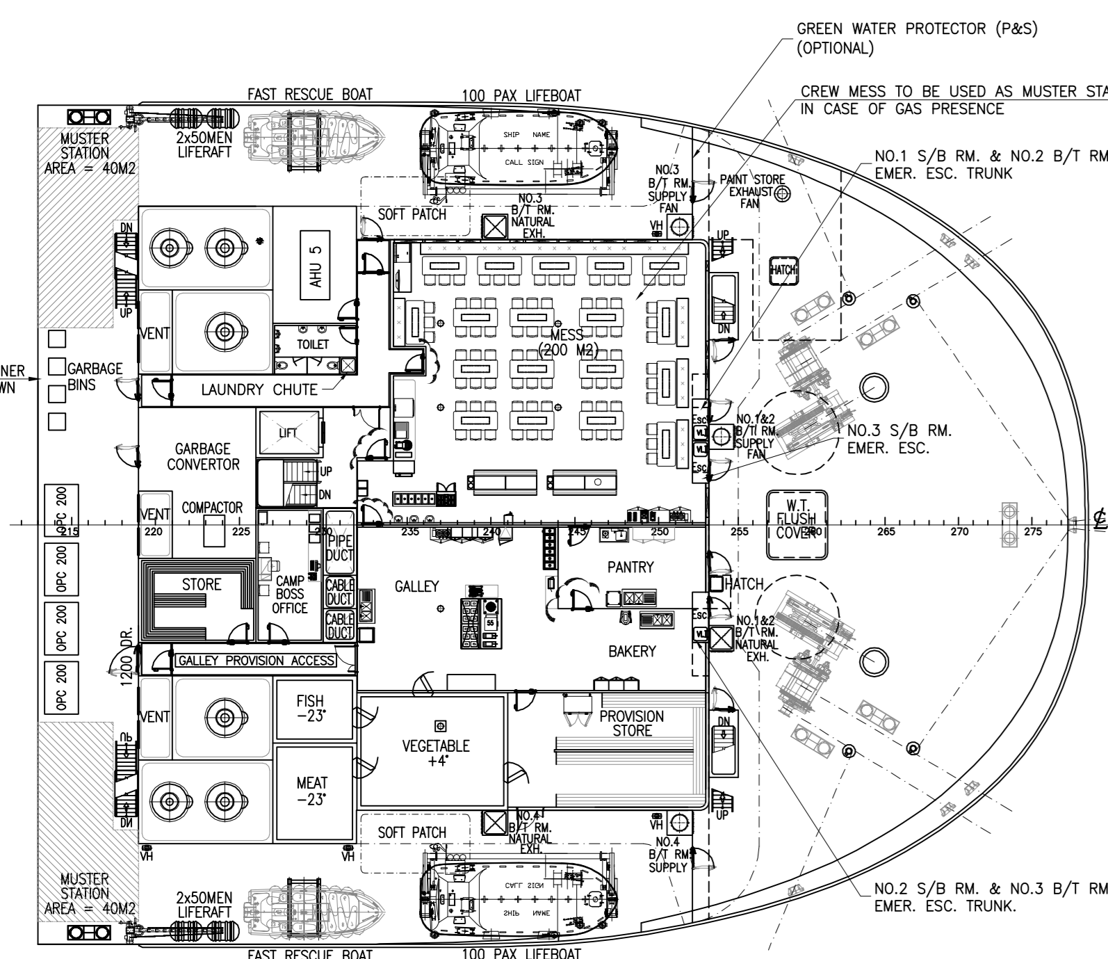
UPPER FORECASTLE DECK
