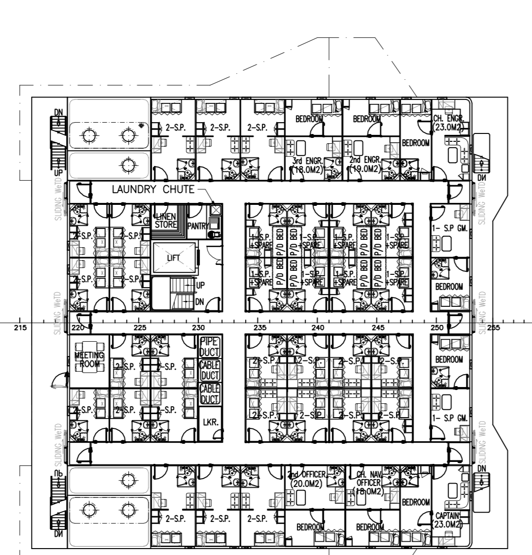
ACCOMMODATION DECK D 6 X 1-CREW = 06 CREW 2 X S.P. GM = 02 S.P. 8 X 1-S.P.+ 1 SPARE = 16 S.P. 23 X 2-S.P. = 46 S.P. TOTAL = 70 PERSONS
