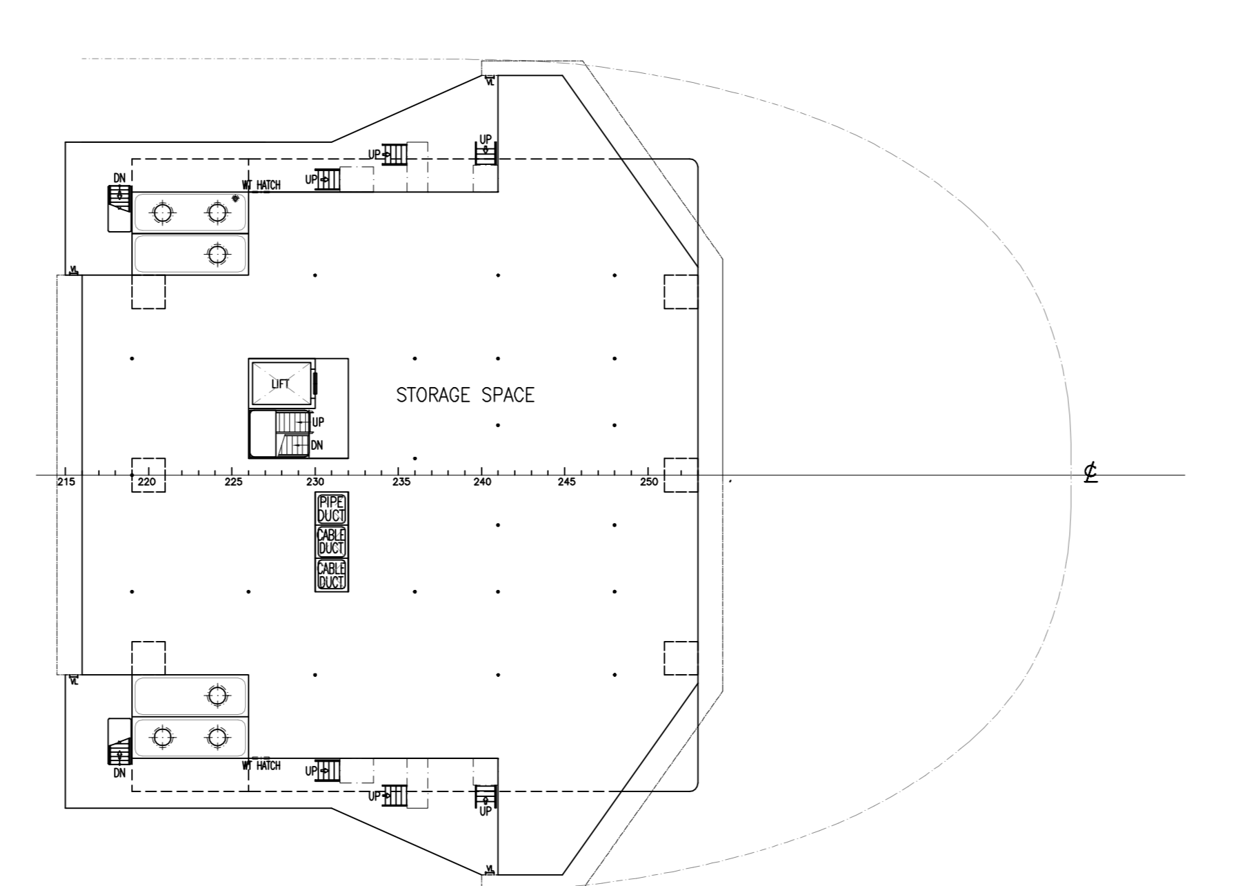
BRIDGE DECK PLAN
