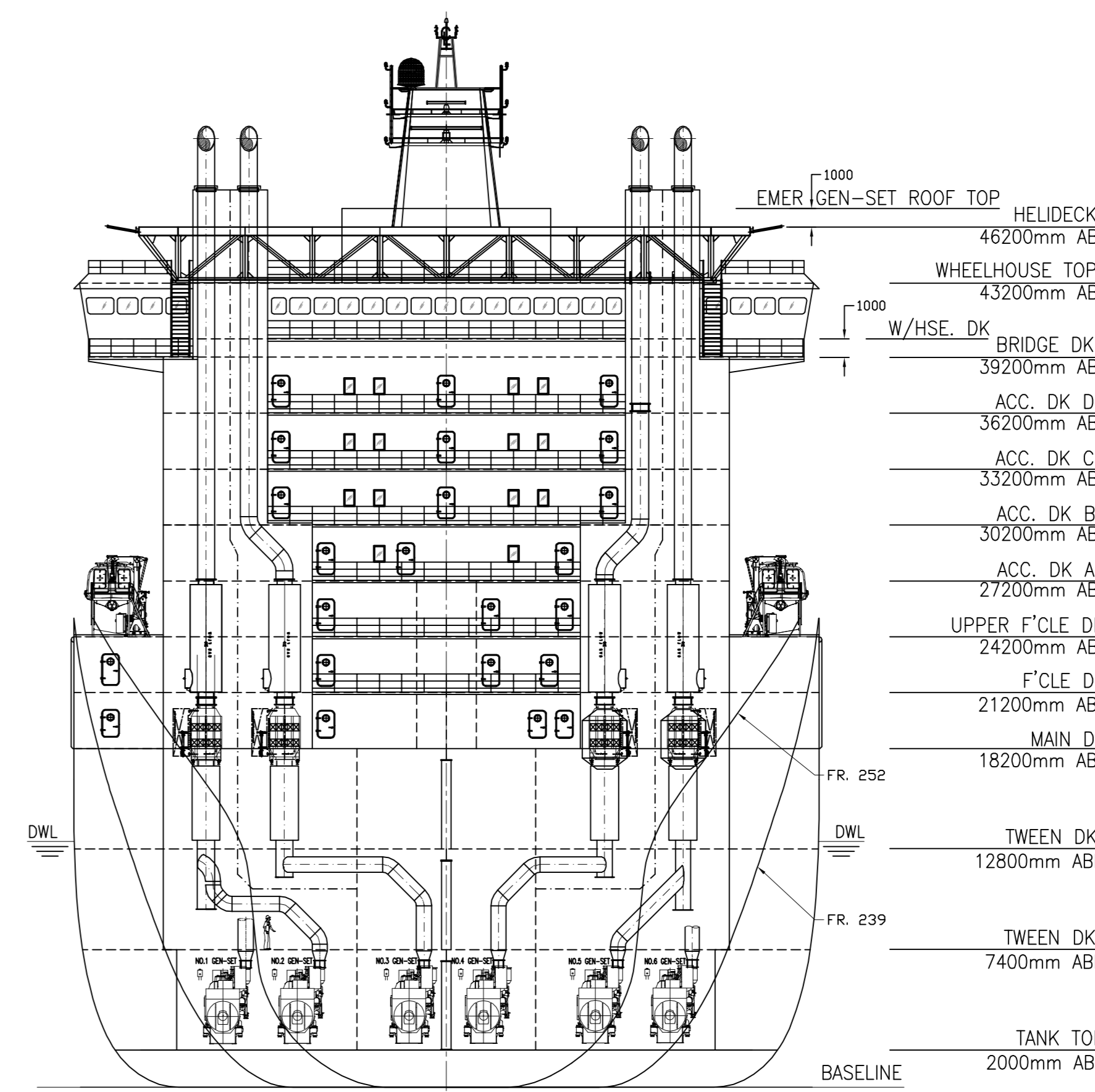
SECTION IWO ENGINE EXHAUST (FRAME 224, LOOKING FWD)
