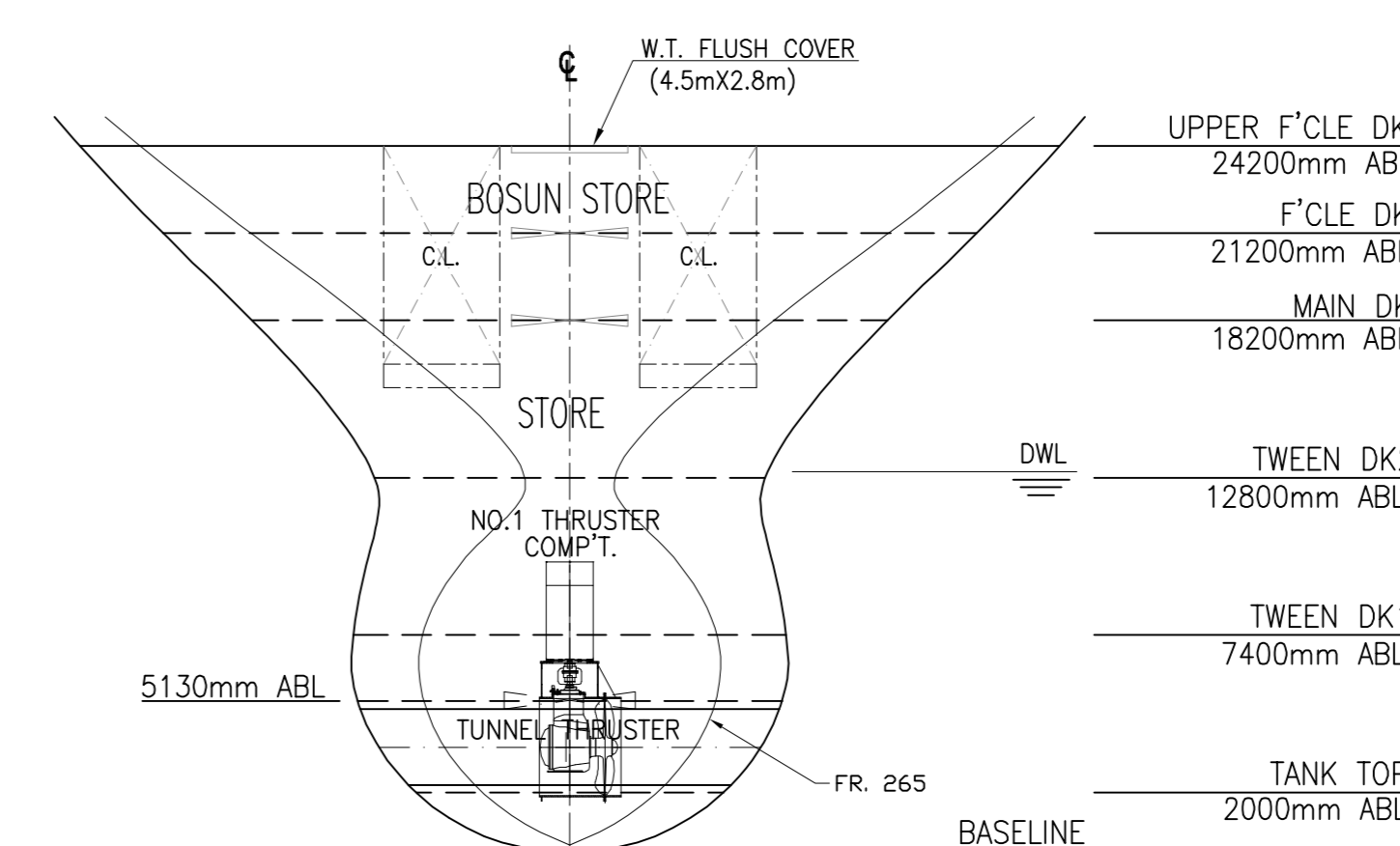
SECTION IWO BOW THRUSTER (FRAME 259, LOOKING AFT)
