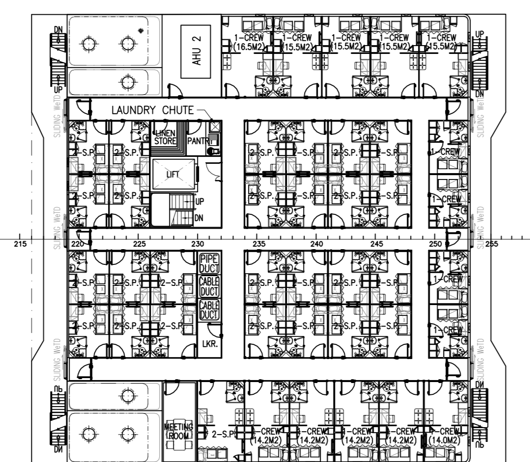
ACCOMMODATION DECK C 14 X 1-CREW = 14 CREW 27 X 2-S.P. = 54 S.P. TOTAL = 68 PERSONS
