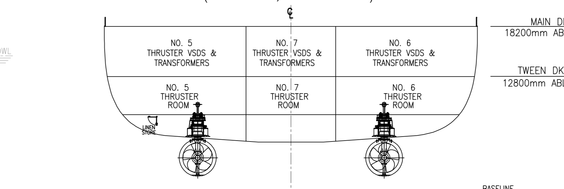
SECTION IWO AFT AZIMUTH THRUSTERS (FRAME 5, LOOKING FWD)
