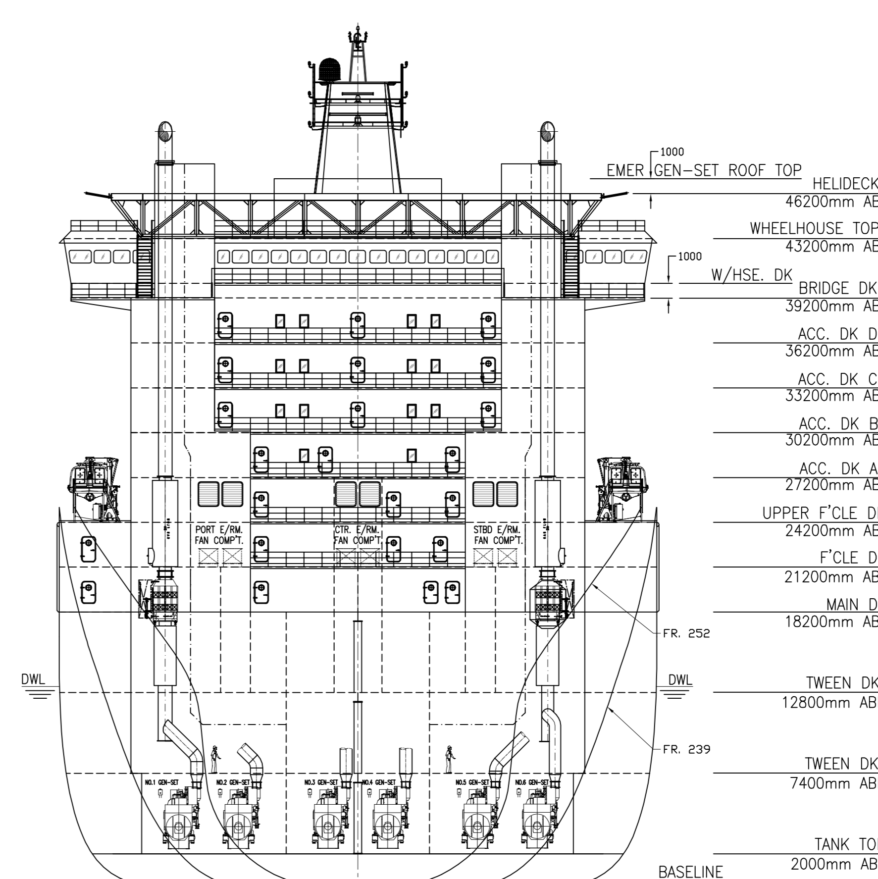
SECTION IWO ENGINE EXHAUST (FRAME 221, LOOKING FWD)
