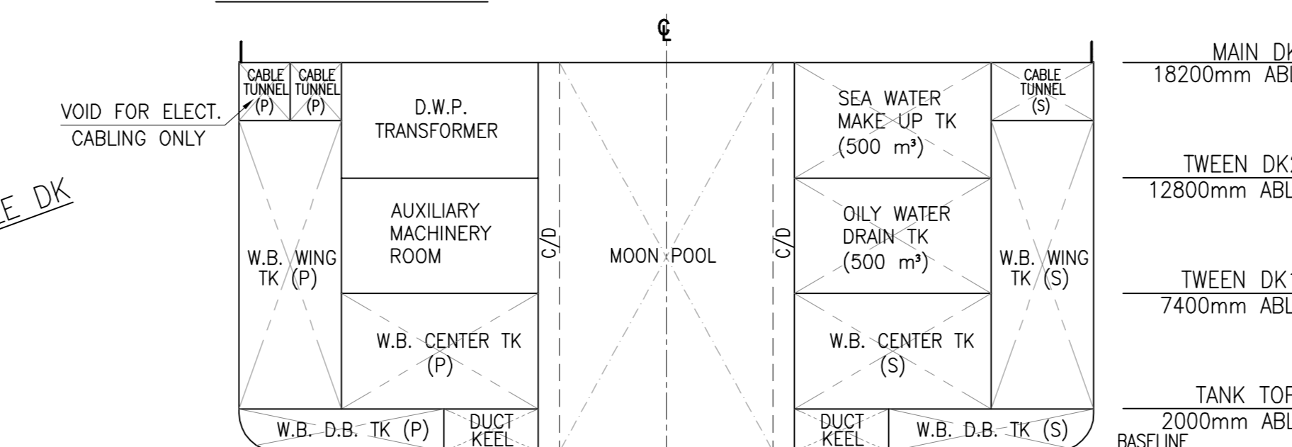
SECTION IWO MOON POOL (FRAME 112, LOOKING FWD)
