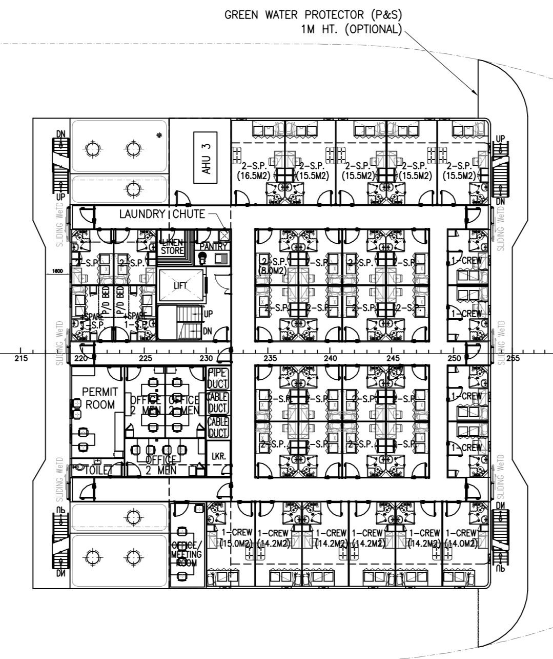
ACCOMMODATION DECK B 10 X 1-CREW = 10 CREW 25 X 2-S.P. = 50 S.P. TOTAL = 60 PERSONS
